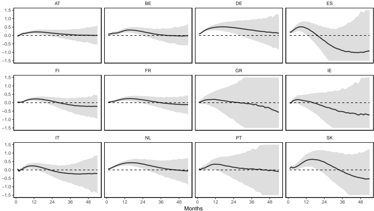
Note: Posterior distribution of impulse responses in percentage points. The median is depicted in grey, the 16 th and 84 th percentile are indicated by the light grey area. The dashed line indicates zero. Country codes may be found in Appendix A .
