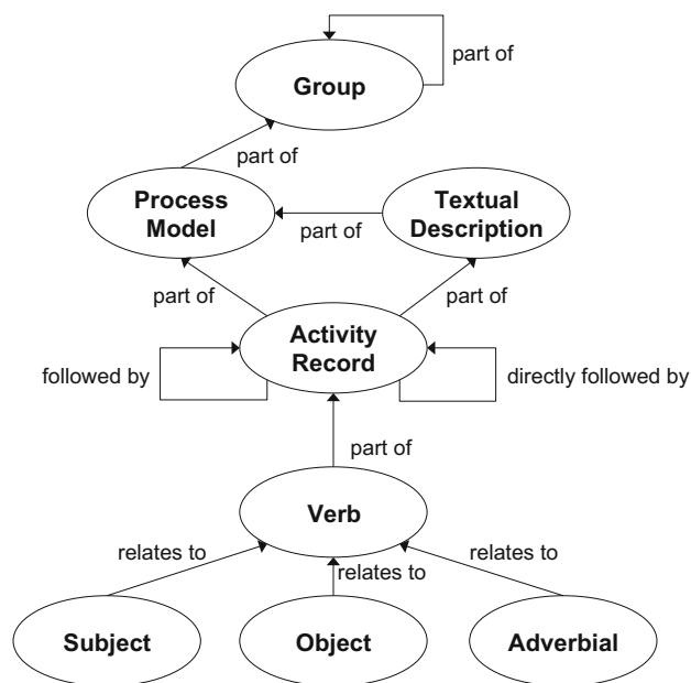
Fig. 3 Overview of unified data format
