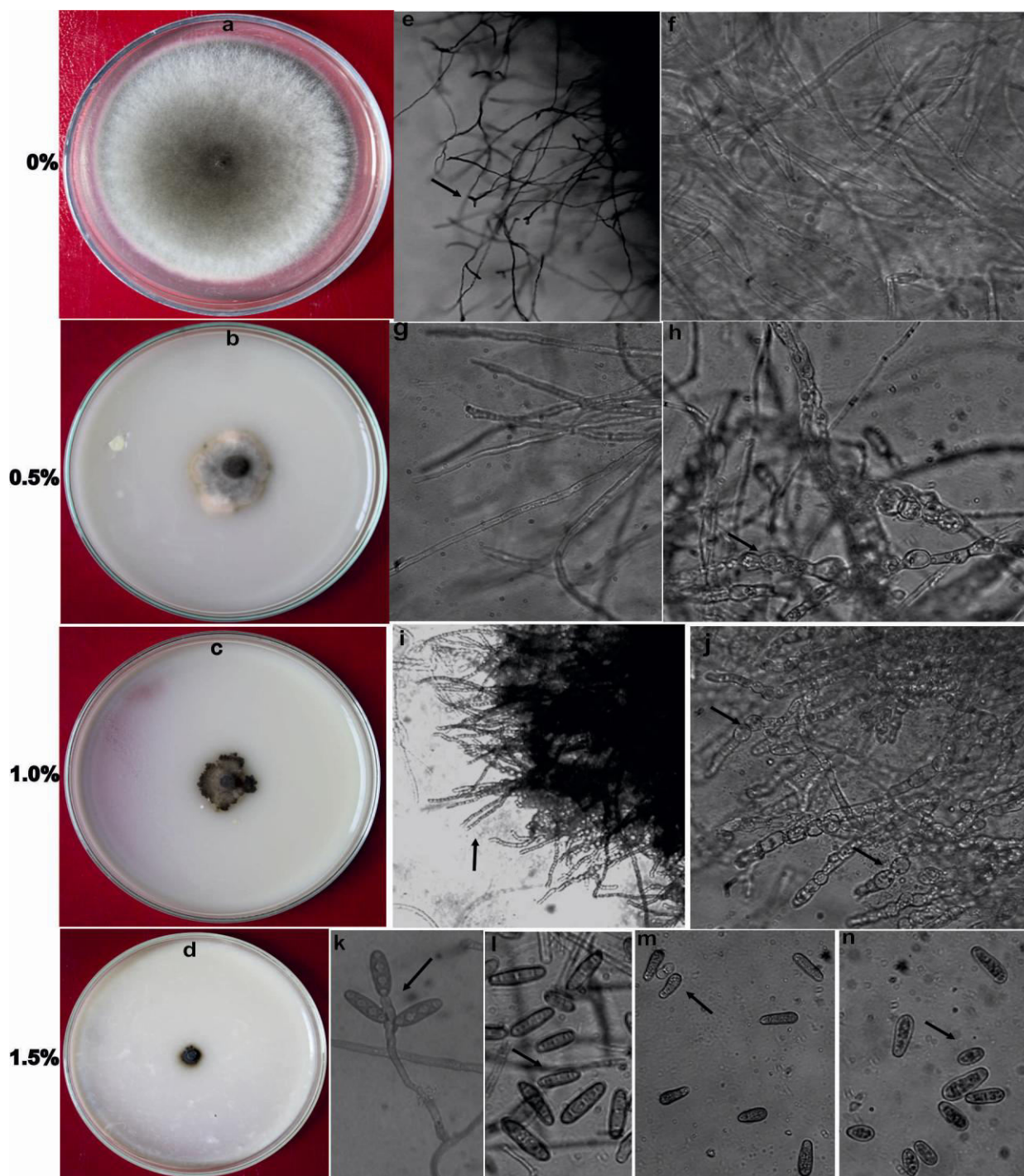
Fig.4: Presenting effect of the different concentrations (0.0, 0.5, 1.0 & 1.5%) of Polyvinylpyrrolidone functionalized zinc peroxide ( ZnO_2 ) nanoparticles supplemented in potato dextrose agar medium six days after inoculation on growth of Bipolaris sorokiniana causing foliar blight of wheat and its spore size; a-d depict significant reduction in growth of the fungus with increase in concentration varying from 0.0-1.5%; e-f depict free normal growth of the fungus at the periphery of fungal colony showing attachment of spores; g-h indicate suppressed fungal growth due to widening and coiling of hyphae with few spores; i-j show excessive beading and coiling of hyphae at 1.0% concentration; k-l exhibit normal size abundant six days young spore with three septa at 0.0% of zinc peroxide and m-n show reduction in spore size at 0.5 and 1.0% of zinc peroxide.
