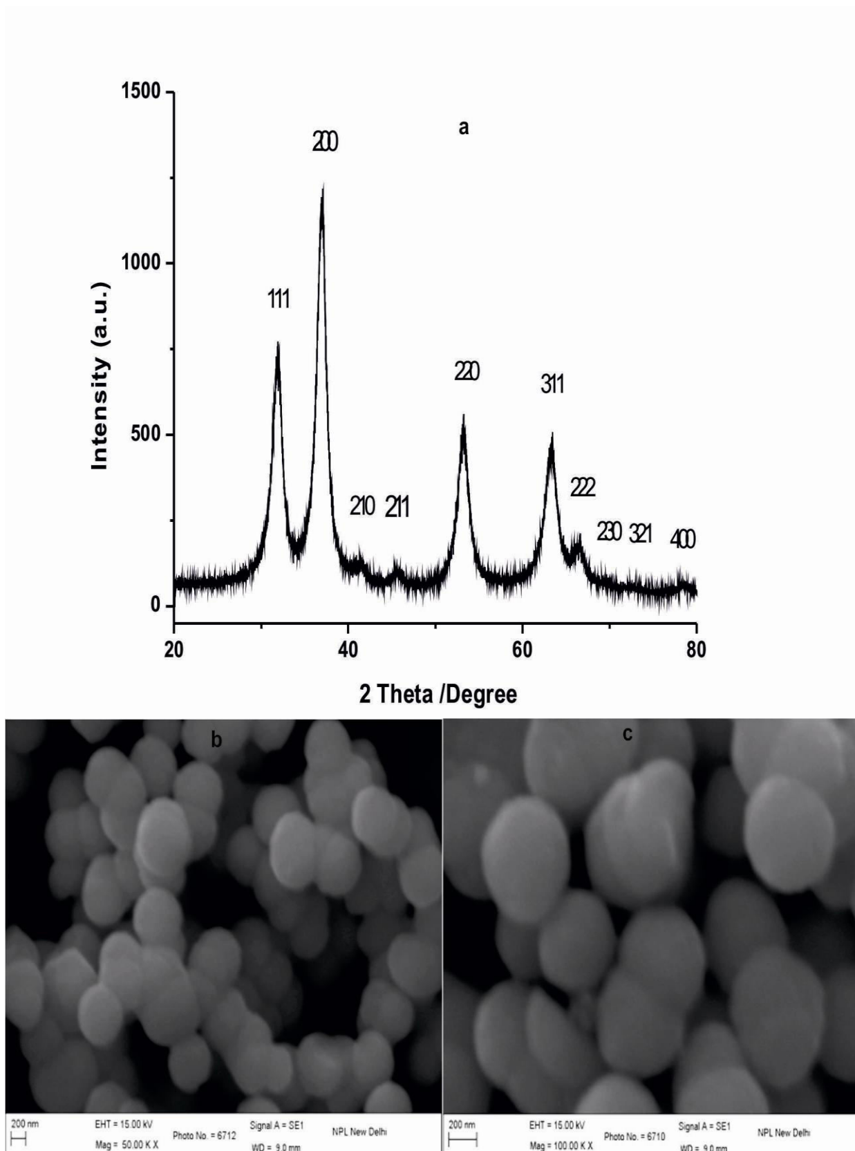
Fig.1: Illustrating characteristics features of Zinc peroxide (ZnO 2 ). a) XRD pattern of ZnO 2 ; b) SEM Micrograph of ZnO 2 at 50 KX magnification and c) SEM Micrograph at 100 KX magnification
