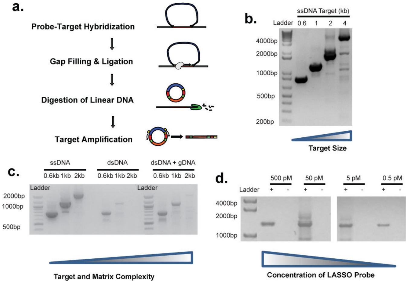
Figure 2. Single ORF target capture with LASSO probes (a) Schematic of single target capture, purification, and amplification. (b) Post capture PCR of circles obtained from the capture of 620 bp, 1 kb, 2 kb, 4 kb target sequences within the M13Mp18 ssDNA genome using 4 different pre-LASSO probes assembled with a 445 bp adapter. (c) Post capture PCR of circles obtained from the capture of 620bp, 1kb, or 2kb sequences using as template ssDNA M13Mp18, dsDNA M13Mp18 amplicon alone, or dsDNA M13Mp18 amplicon in a background of 10 pM sheared E. coli K12 genomic DNA. (d) Post capture PCR of circles obtained by capturing a 1,038 bp target sequence within the M13Mp18 dsDNA (~500 fM) in presence of an equimolar (~500 fM) background of total genomic DNA of E. coli , using serial dilution of a LASSO probes. Negative controls contain sheared gDNA but no target.
