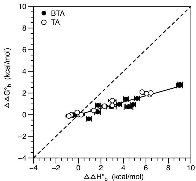
Figure 4. The influence of mutations on binding affinity. Circles plot the influence of mutations on the free energy of binding against their influence on the enthalpy of binding ( \Delta\Delta G_{b=mut}^\circ against \Delta\Delta H_{b=mut}^\circ from Fig. 2A). The black line through these points represents a linear fit (slope = 0.29 and R^2 = 0.90 ; n \geq 7 ; error bars represent standard error). Mutations that increase the enthalpic cost of binding lower binding affinity (i.e., make \Delta G_b^\circ more positive).
