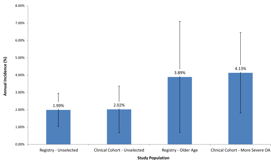
Fig. 2 Mean Annual Incidence of Registry – Unselected, Clinical Cohort – Unselected, Registry – Older Age, and Clinical Cohort – More Severe OA. Each bar represents the estimated yearly incidence of TKA from the logistic random effects model. The vertical lines represent the 95% confidence intervals
