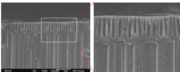
Figure 8. The cross section SEM image of the top aluminum foil under the leakage blocking experiment
