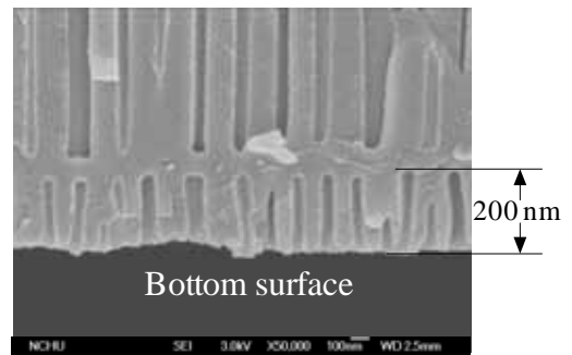
Figure 4. Bi-directional porous pattern growing from both the top and bottom surfaces
