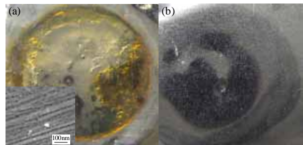
Figure 10. SEM images of the triplex foils laminate experiment (a) Middle foil (b) Bottom foil
