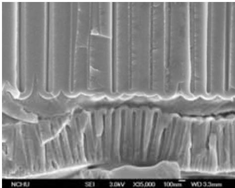
Figure 12. The cross section SEM image of the nano-capsule array
