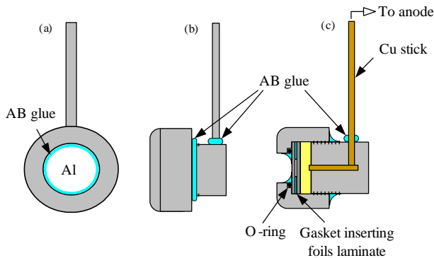
Figure 7. Schematic illustration of the fixture sealing arrangements (a)Front view (b)Side view (c)Cross section view
