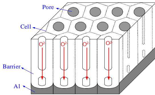
Figure 11. Oxygen ions penetrating mechanism
