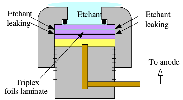
Figure 9. Triplex foils laminate
