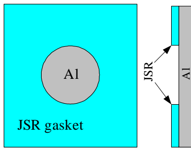
Figure 6. Spin-coated and photolithographic patterned JSR gasket
