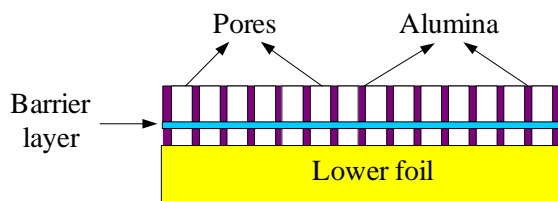
Figure 2. Anodized aluminum foils
