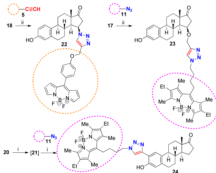
Scheme 5. Reagents and conditions: (i) CuI (0.05 equiv.), Ph 3 P (0.1 equiv.), DIPEA (3 equiv.), 1 equiv. TBAF, toluene, reflux, 2 h; (ii) CuI (0.05 equiv.), Ph 3 P (0.1 equiv.), DIPEA (3 equiv.), toluene, reflux, 2 h.
