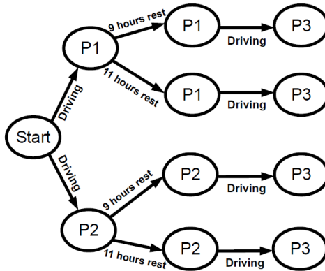
Figure 1: An example subtree of the algorithm
