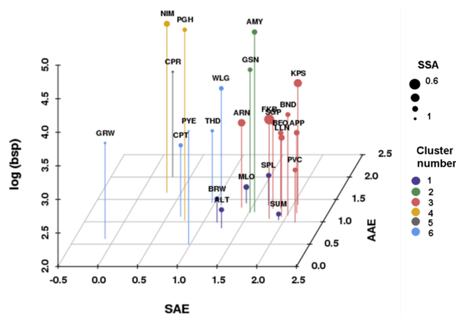
Figure 3. Three-dimensional parameter space of SAE vs. AAE vs. \log of scattering coefficient, \sigma_{sp} ( \text{Mm}^{-1} ). Station points are colored by cluster number resulting from the clustering analysis and sized by median SSA value.
