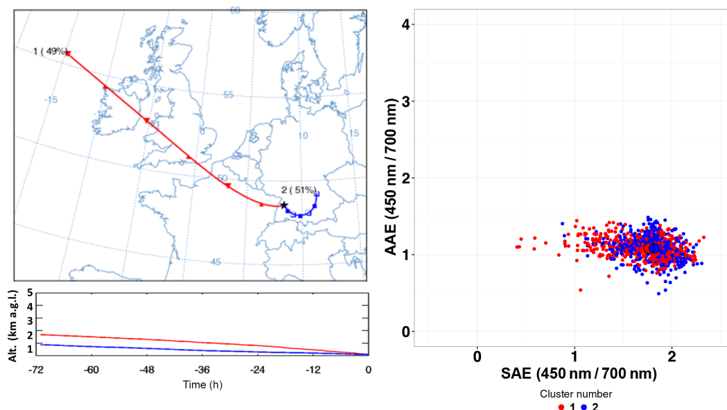
Figure 7. Back trajectory map, back trajectory height (in kilometers above ground level) vs. time and AAE vs. SAE plot space for the Black Forest, Germany, station FKB, all color-coded by back trajectory cluster number.
