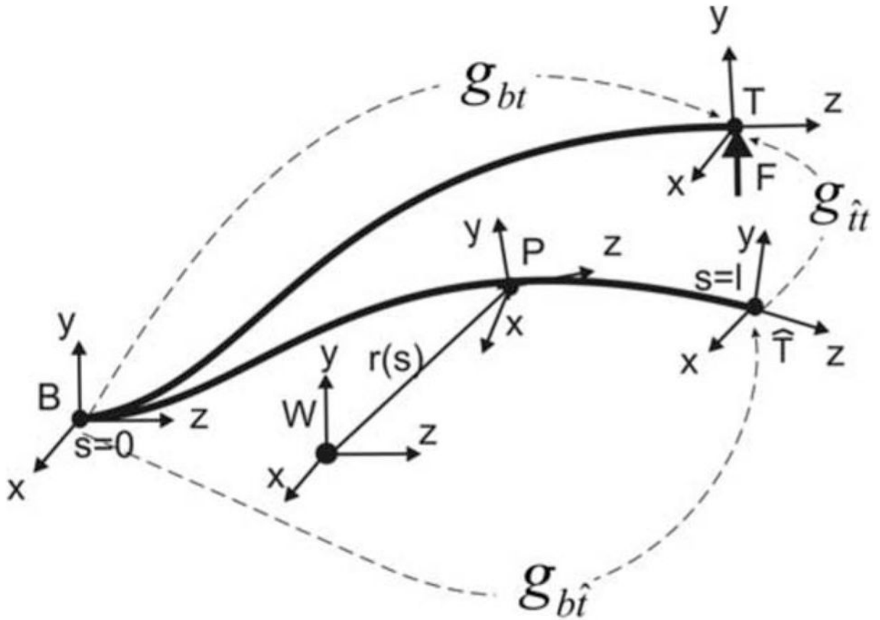
Fig. 3. Continuum robot represented as a space curve (solid line). W is world coordinate frame, while B , P , T , and \hat{T} are robot body frames. T and \hat{T} are tip frames without and with the application of tip wrench F , respectively. Coordinate transformations are denoted by g_{bt} , g_{b\hat{t}} and g_{\hat{t}t} .
