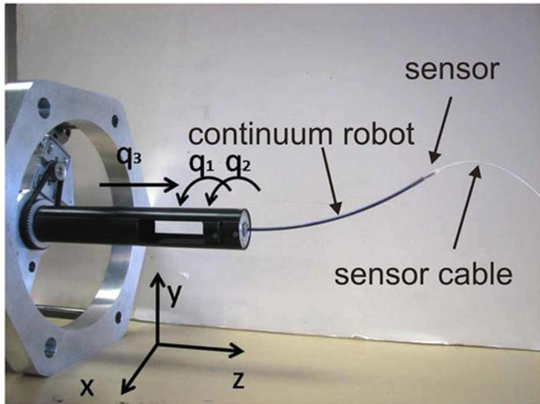
Fig. 7. Concentric tube manipulator mounted in its drive system. Electromagnetic sensor is shown attached to robot tip. Actuator variables q_1 and q_2 control rotation of two tubes and q_3 controls translation of tube pair. Curvature is varied by relative rotation of the tubes.
