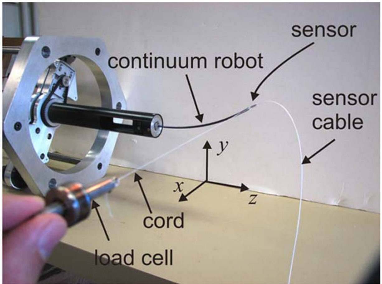
Fig. 8. Interaction with a moving environment. Environment motion is produced by manual loading of the robot tip through a cord attached to a load cell.
