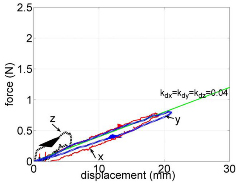
Fig. 11. Tip force versus displacement in the three coordinate directions for a noncontact robot curvature of u^w = [(1/320 \text{ mm}) \ 0 \ 0]^T and desired tip stiffness of K_d = \text{diag}(0.04 \ 0.04 \ 0.04) N/mm.
