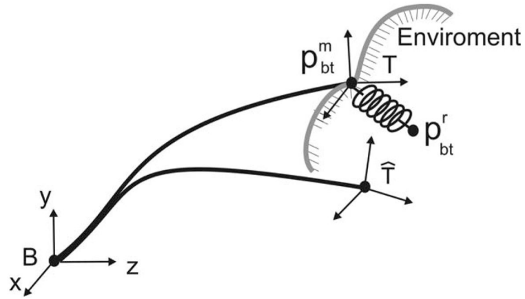
Fig. 4. Robot in contact with environment. The stiffness controller implements a virtual linear spring at the robot's tip. Desired actuator positions are such that when robot is deflected from unloaded tip configuration T to configuration T , the desired tip spring force is generated, and the desired tip orientation is achieved.
