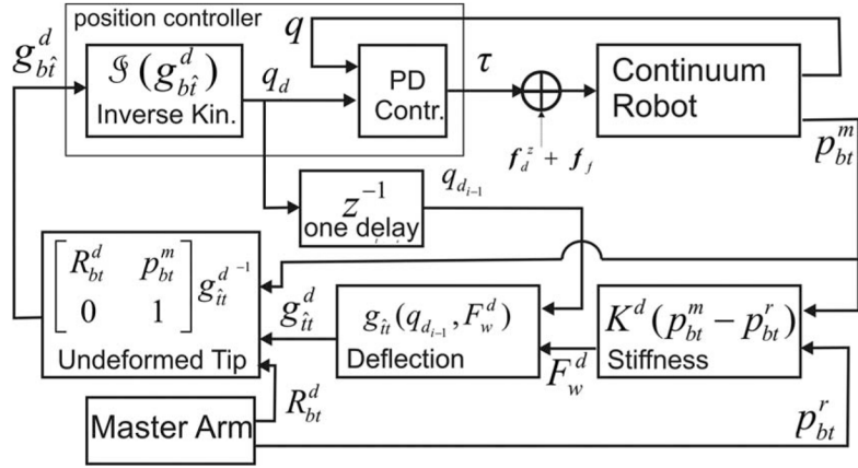
Fig. 5. Block diagram of the stiffness controller. A single fixed-point iteration is performed per controller cycle.
