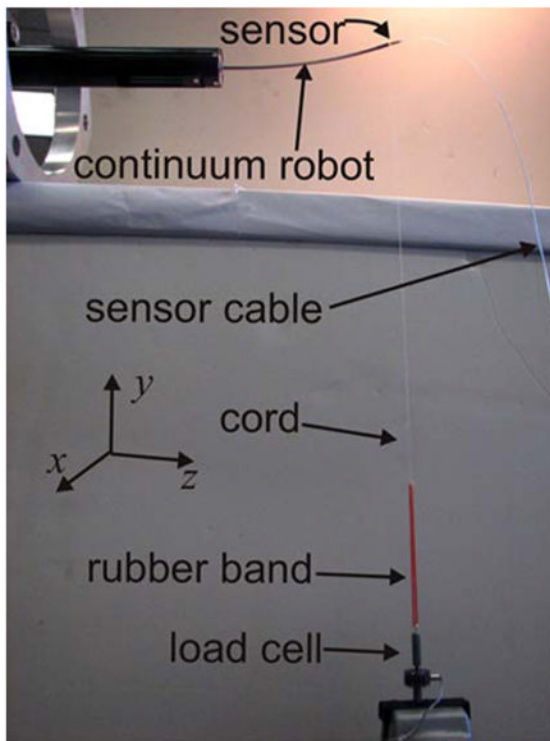
Fig. 9. Interaction with a fixed elastic environment. Environment is modeled by a rubber band connecting a tip-mounted cord and a fixed load cell.
