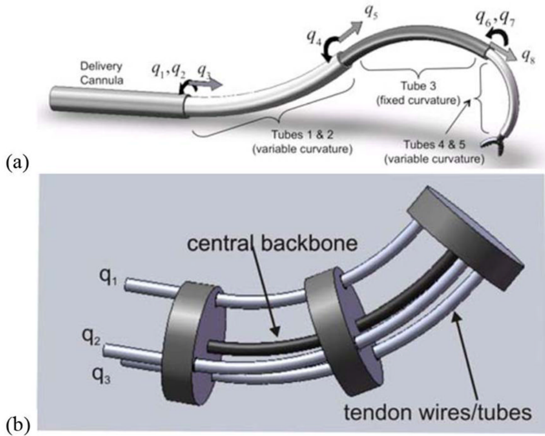
Fig. 2. Schematics of two types of continuum robots. (a) Concentric tube robot. (b) Tendon-driven robot with flexible backbone.
