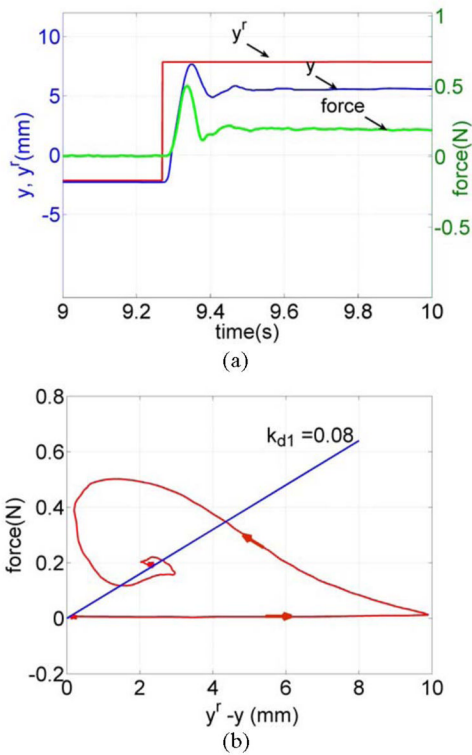
Fig. 14. Stiffness controller step response. Step change in reference position y^r is applied such robot transitions from free space to contact with environment through cord. Desired stiffness is k_d = 0.08 N/mm. (a) Time response plot of y^r , y , and f_y . (b) Tip force versus virtual spring displacement y^r - y .
