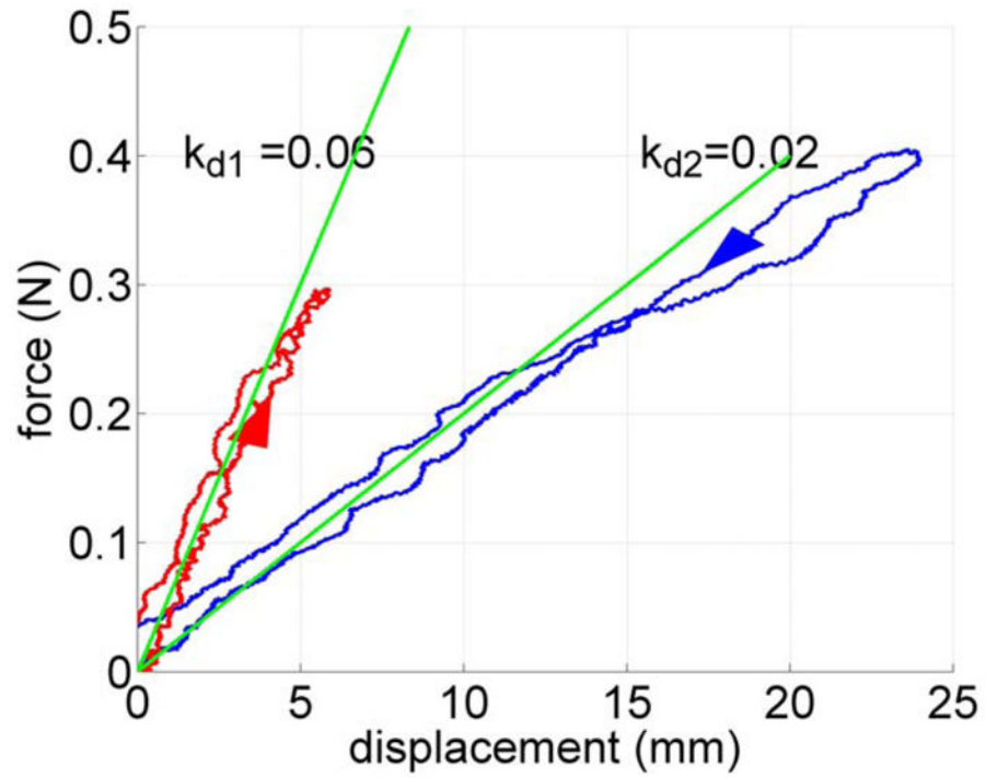
Fig. 13. Tip force versus displacement in the y -direction during contact with a soft stationary environment for desired stiffness values of 0.02 and 0.06 N/mm.
