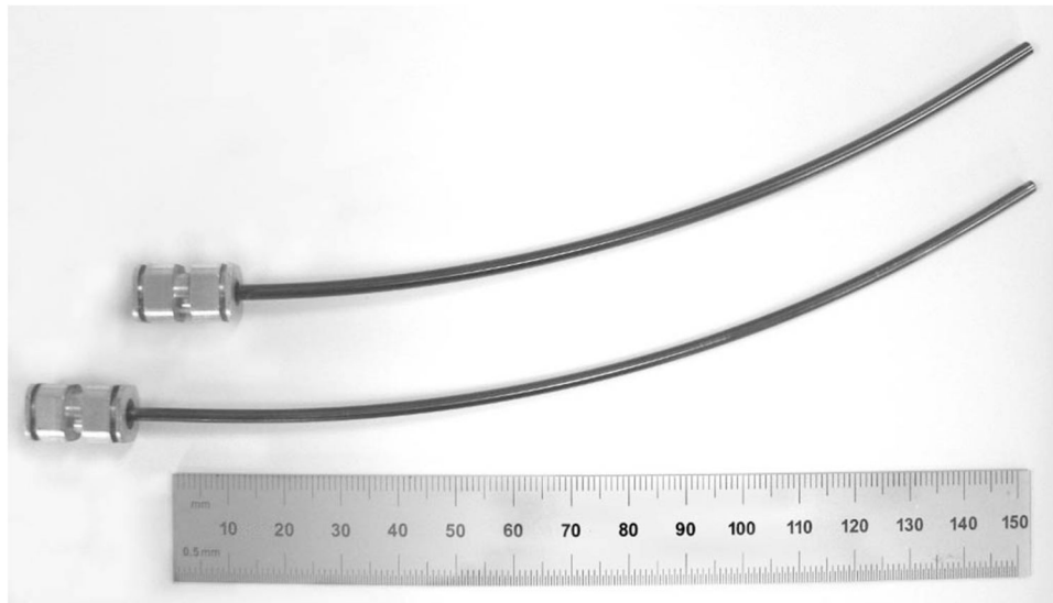
Fig. 6. Robot component tubes. NiTi tubes assemble concentrically to form a 3-DOF robot. Tubes are of equal initial curvature and bending stiffness. The outer tube (top) has an outer diameter of 2.8 mm and inner diameter of 2.5 mm. The inner tube (bottom) has an outer diameter of 2.4 mm and an inner diameter of 2.0 mm.
