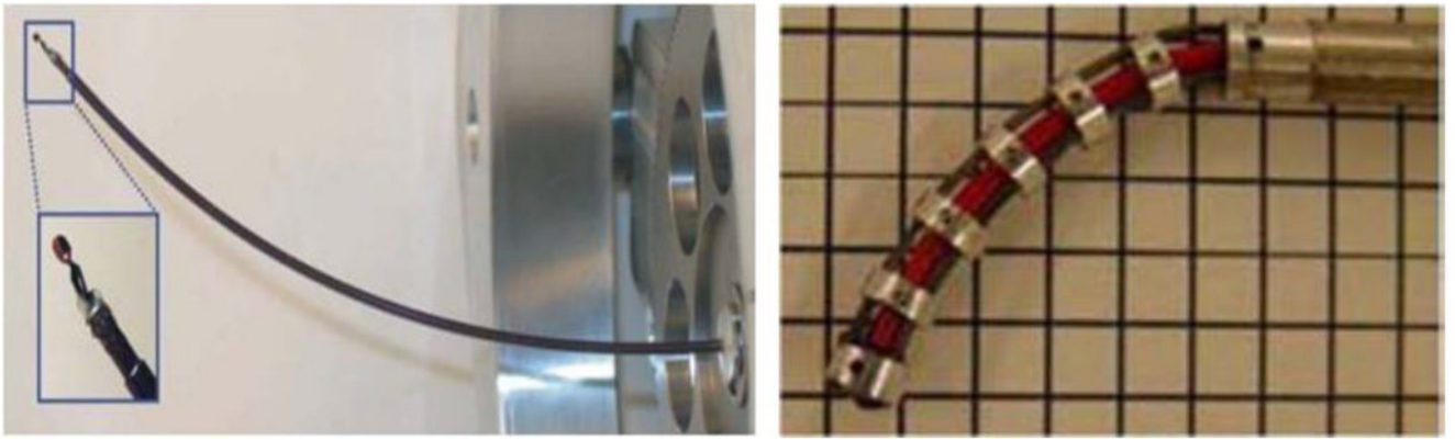
Fig. 1. Examples of continuum manipulators. (a) Twenty-centimeter-long concentric tube robot with 1-mm-wide tip-mounted forceps. (b) Four-millimeter diameter multi-backbone robot [4].
