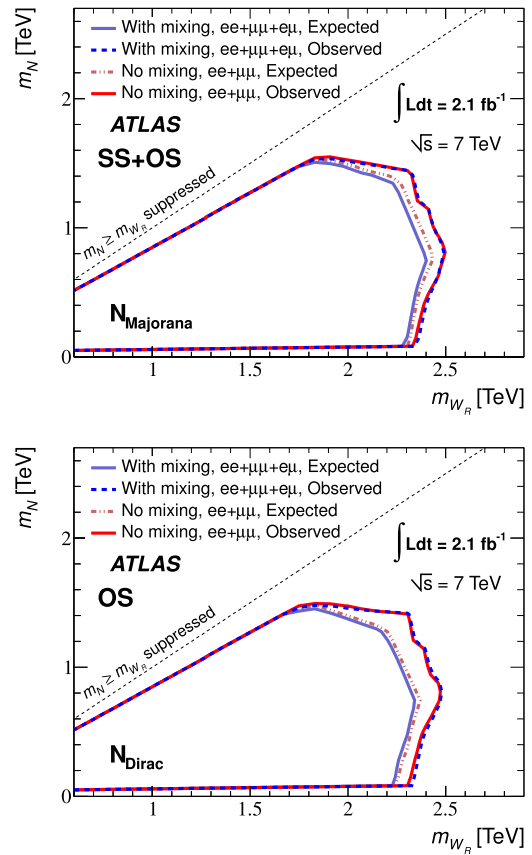
Fig. 4 Expected and observed 95 % C.L. upper limits on the heavy neutrino and W_R masses for the Majorana (top) and Dirac (bottom) cases, in the no-mixing and maximal-mixing scenarios
