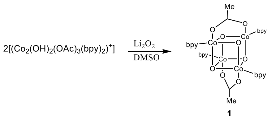
Figure 6.1. Synthesis of the Christou-cube by condensation of two cobalt dimers.
