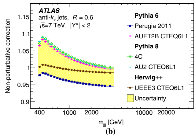
Fig. 2 Non-perturbative corrections obtained using various MC generators and tunes for the differential three-jet cross-section as a function of three-jet mass in the range |Y^*| < 2 for anti- k_r jet a R = 0.4 and b R = 0.6
