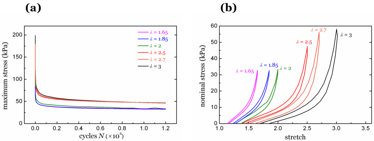
Fig. 2 (a) The maximum stress in each cycle decreases and approaches a steady state. (b) The stress-stretch curves after 2000 cycles for different maximum stretches \lambda .
