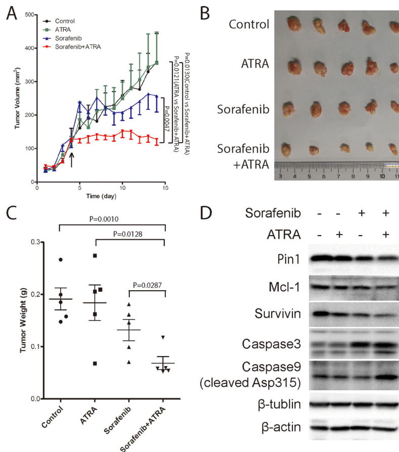
Figure 7: The Pin1 inhibitor ATRA synergistically enhances the ability of sorafenib to inhibit tumor growth of HCC in vivo . (A) Tumor growth was significantly inhibited by the combination of sorafenib and ATRA. Huh7 cells were injected subcutaneously into nude mice. Drugs were administrated when tumors at the point indicated by the arrow. 1/4 tablet of 10 mg 21 day slow-releasing ATRA pellet was inoculated subcutaneously. Sorafenib (40 mg/kg) was orally given every three days. Tumor growth was measured every 3 days, and tumor volume was calculated using the formula of length*width*width/2. (B, C) ATRA synergistically enhanced sorafenib anti-tumor effect in vivo . Tumors were harvested (B) and weighted (C) when the length of largest tumor reached 1.0 cm. (D) ATRA synergistically enhanced sorafenib induced Pin1 down-regulation in vivo . Pin1, Mcl-1, survivin, beta-actin, beta-tubulin, cleaved caspase 9 and caspase 3, protein expressions were determined by Western Blot.
