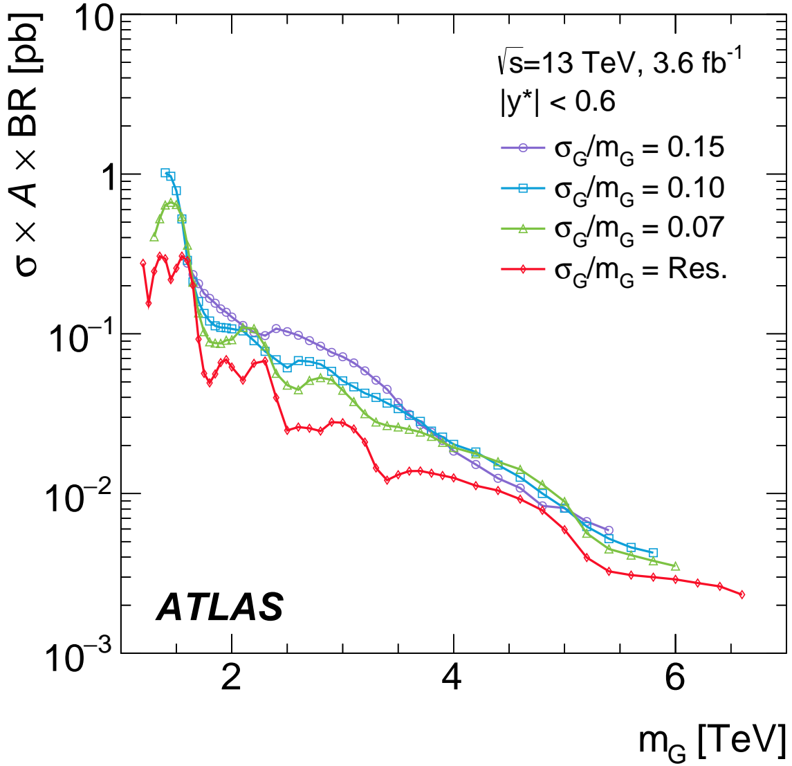
Figure 5: The 95% credibility-level upper limits obtained from the m_{jj} distribution on cross-section times acceptance times branching ratio to two jets, \sigma \times A \times BR , for a hypothetical signal with a cross-section \sigma_G that produces a Gaussian contribution to the observed m_{jj} distribution, as a function of the mean mass of the Gaussian distribution, m_G . Limits are obtained for four different widths, from a width equal to the detector mass resolution (“Res.”), 3%–2% depending on m_{jj} probed, to 15% of the mean of the Gaussian mass distribution.
