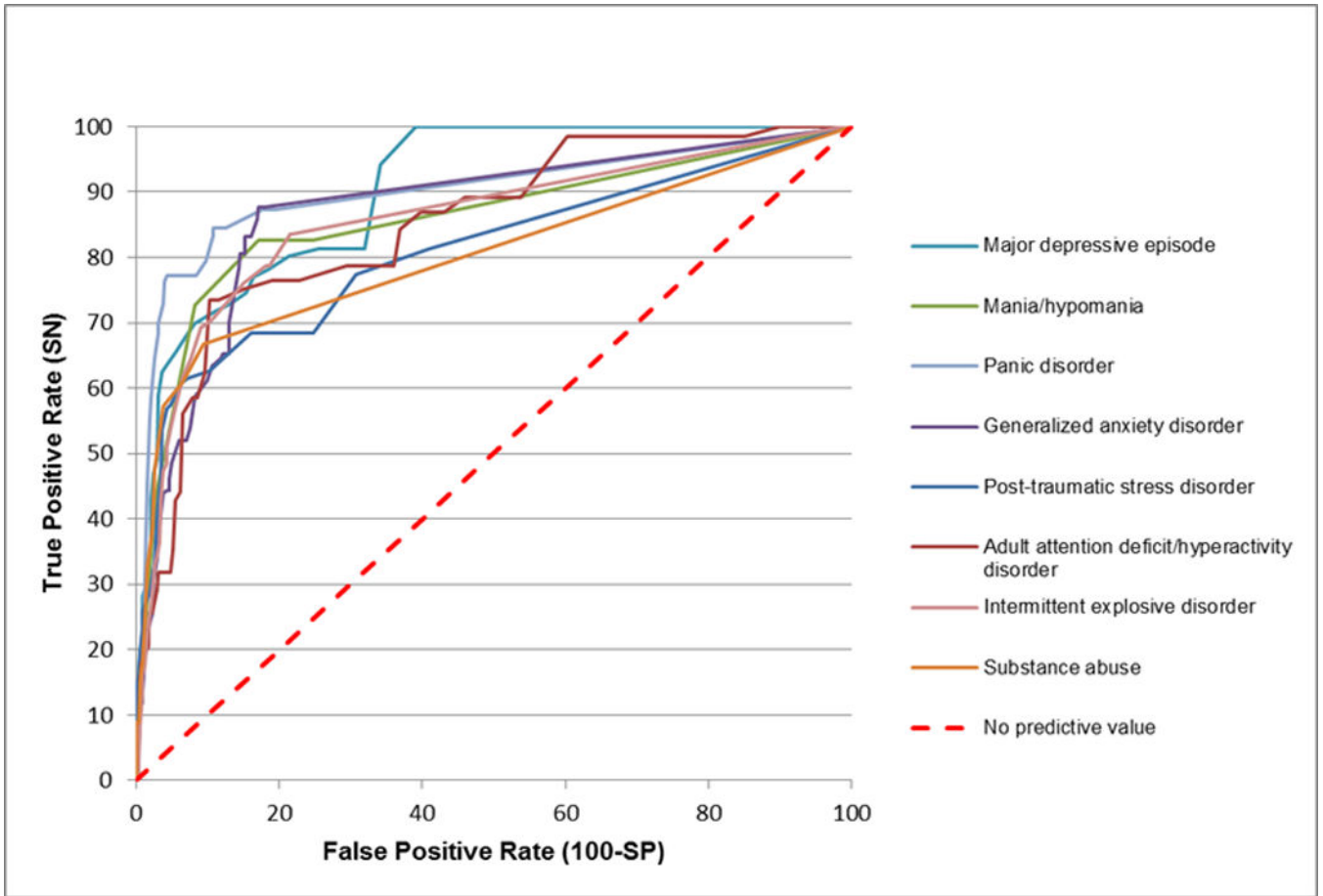
Figure 1. ROC curves for the associations between continuous screening scales and DSM-IV/SCID diagnoses (n=460) a
