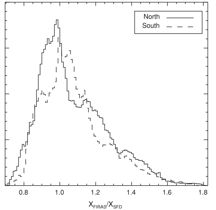
Figure 22. Ratio X_{\text{FIRAS}}/X_{\text{SFD}} in the north (solid) and in the south (dashed). The temperature correction is systematically higher in the south than in the north by \sim 10\% , about compatible with the difference in best-fit normalization between the north and south found in Section 4.3.
