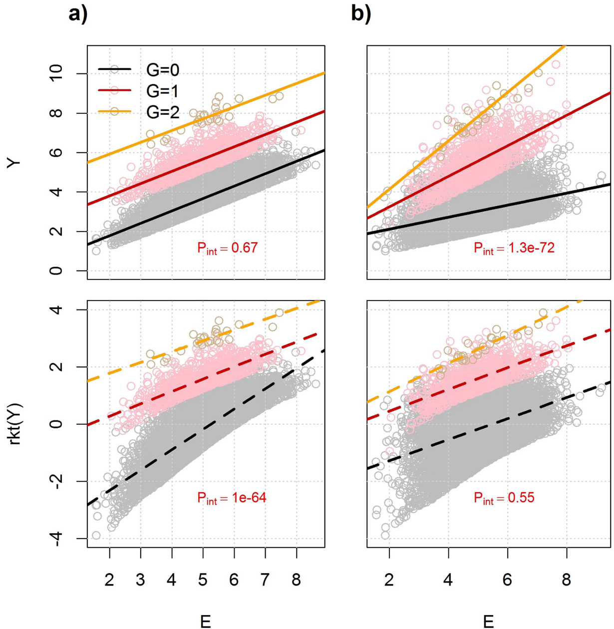
Fig 2. Effect of non-linear transformation on interaction effects. We defined an outcome Y as a function of a single nucleotide polymorphism G with a minor allele frequency of 0.1, an exposure E normally distributed with mean 5 and variance 1, and a right-skewed normal distributed residual term \epsilon . In the framework of this analysis, TF mRNA level is considered as an exposure E . We generated two datasets of 10,000 individuals for the two scenarios. In a) G and E have only main effects and each explain 20% of the variance of Y . In b) G and E main effects each explain 10% of the outcome variance, but also have an interaction effect explaining 20% of the variance of Y . Upper panels show Y as a function of E by genotypic class and trend slope from a standard linear regression. Lower panels show the same data plotted after a rank-normal transformation ( rkt ) of Y . Interaction effect (observed as differences in slope by genotypic class) appears or disappears depending on the transformation applied to Y . P -values for interaction are indicated in red.
