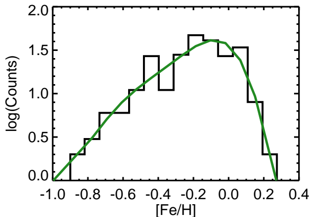
FIG. 1.— Logarithmic number of stars versus logarithmic metallicity bin. The black histogram displays the distribution of metallicities in the Casagrande et al. (2008) sample and the green line is our adopted metallicity prior.
