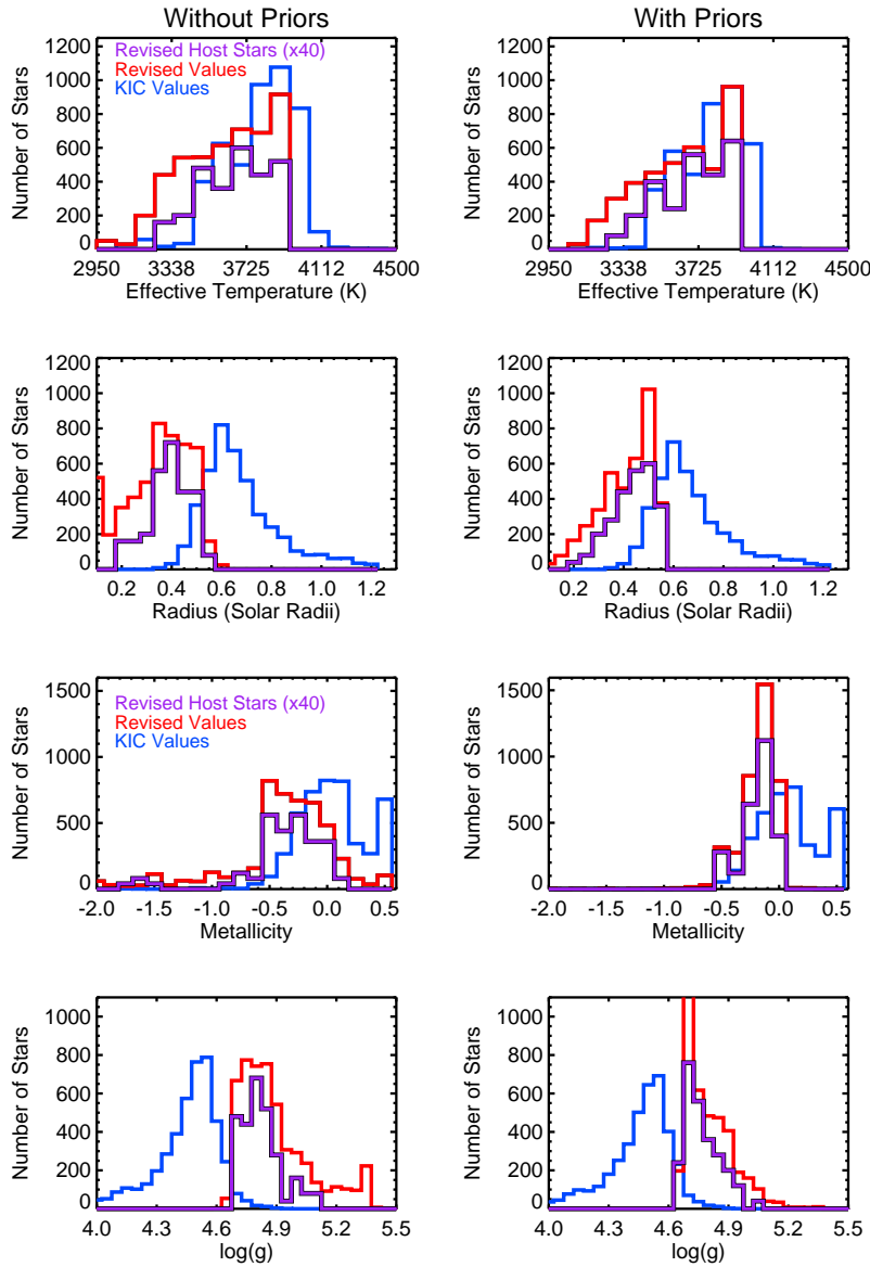
FIG. 3.— Histograms of the resulting temperature (top), radius (second from top), metallicity (third from top), and surface gravity (bottom) distributions for the target stars with revised temperatures below 4000K. The panels on the left show the distributions resulting from fitting the stars without setting priors while the stellar parameters in the right panels were fit assuming priors on metallicity and height above the plane. In all panels, a histogram of the original KIC values is shown in blue and a histogram of the revised values is plotted in red. The distribution of cool host stars (multiplied by forty) is shown in purple in all plots.
