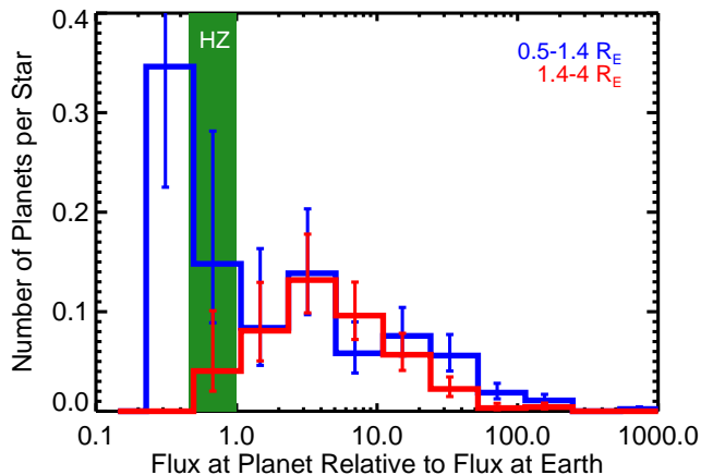
FIG. 19.— Planet occurrence rate versus insolation for Earth-size planets ( 0.5-1.4 R_{\oplus} , blue) and 1.4-4 R_{\oplus} planets (red). The green box marks the habitable zone. The error bars indicate the errors from binomial statistics and do not include errors from the stellar and planetary radius estimates although we do consider those errors as discussed in Section 5.7.
