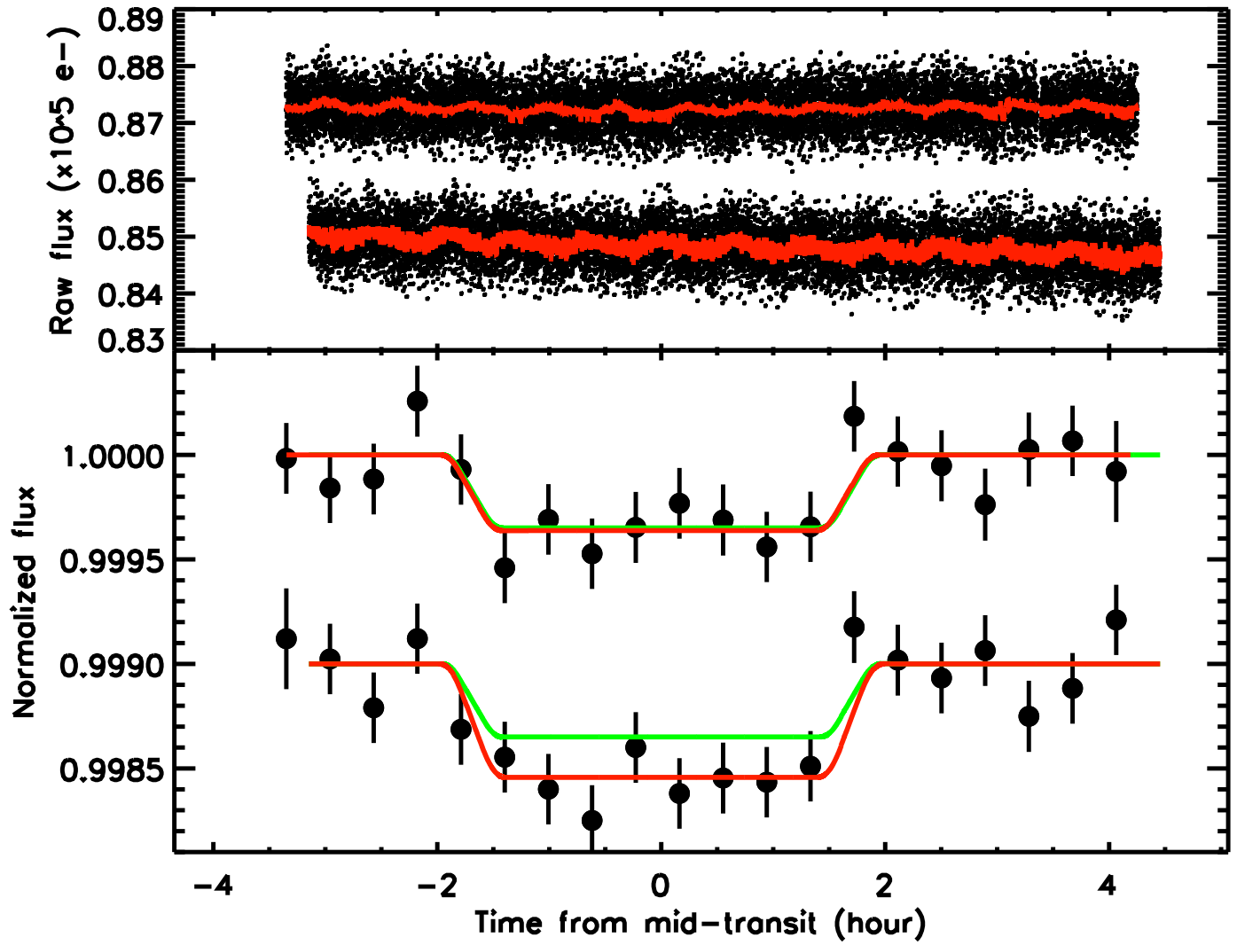
FIG. 9.— Spitzer transit light-curves of Kepler-68b observed in the IRAC band-pass at 4.5 \mu\text{m} . Top panel : raw (unbinned) transit light-curves for the two visits of Kepler-68b. The second visit (at the bottom) is shifted vertically from the first visit (at the top) for display purpose. The red solid lines correspond to the best fit model which include the time and position instrumental decorrelations as well as the model for the planetary transit (see text). Bottom panel : corrected, normalized, and binned by 23 minutes transit light-curves with the transit best-fit plotted in red and the transit shape expected from the Kepler observations overplotted as a green line. The second visit has again been shifted down for display.
