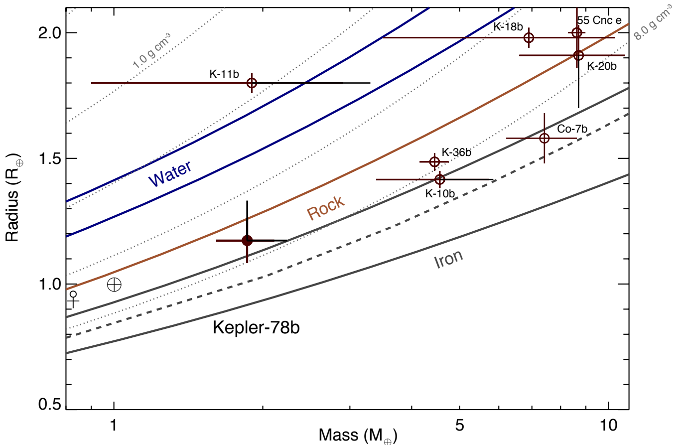
Figure 3 - The hot, rocky planet Kepler-78b placed on a planetary mass–radius diagram. Here masses and radii represent the modes of the corresponding distributions derived from the MCMC analysis, and the error bars represent the 68.3% confidence interval ( 1\sigma ). For comparison, Earth and Venus are indicated in the same diagram by corresponding symbols. The other exoplanets shown are those for which mass and radius have been estimated (K, Kepler; Co, CoRoT). From top to bottom, the solid lines show mass and radius for planets consisting of pure water, 50% water, 100% silicates, 50% silicates and 50% iron core, and 100% iron, as computed with the theoretical models of ref. 18. The dashed line shows the maximum mantle-stripping models from ref. 21; that is, Earth-like exoplanets made of pure iron are not expected to form around normal stars. From top to bottom, the dotted lines represent mean densities of 1, 2, 4 and 8 \text{ g cm}^{-3} .
