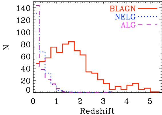
FIG. 1.— Redshift distribution for all 1242 spectroscopically identified ChaMP extragalactic sources.
