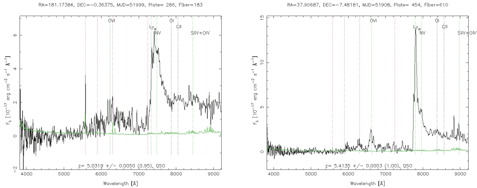
FIG. 16.— SDSS optical spectra of the two highest redshift objects found in our sample. They both are broad-line X-ray QSOs at z > 5 .
