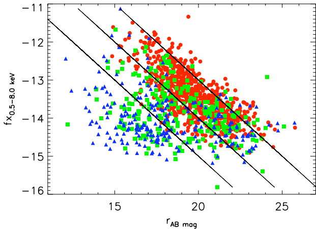
FIG. 7.— Broad-band X-ray flux in logarithmic scale versus r-band magnitude for all our 1242 extragalactic sources. Red circles, green squares and blue triangles denote broad-line AGN, narrow emission line and absorption line galaxies respectively. Line of constant X-ray-to-optical flux ratio (0.1, 1, 10) are given by Equation 1 of Szokoly et al. (2004).
