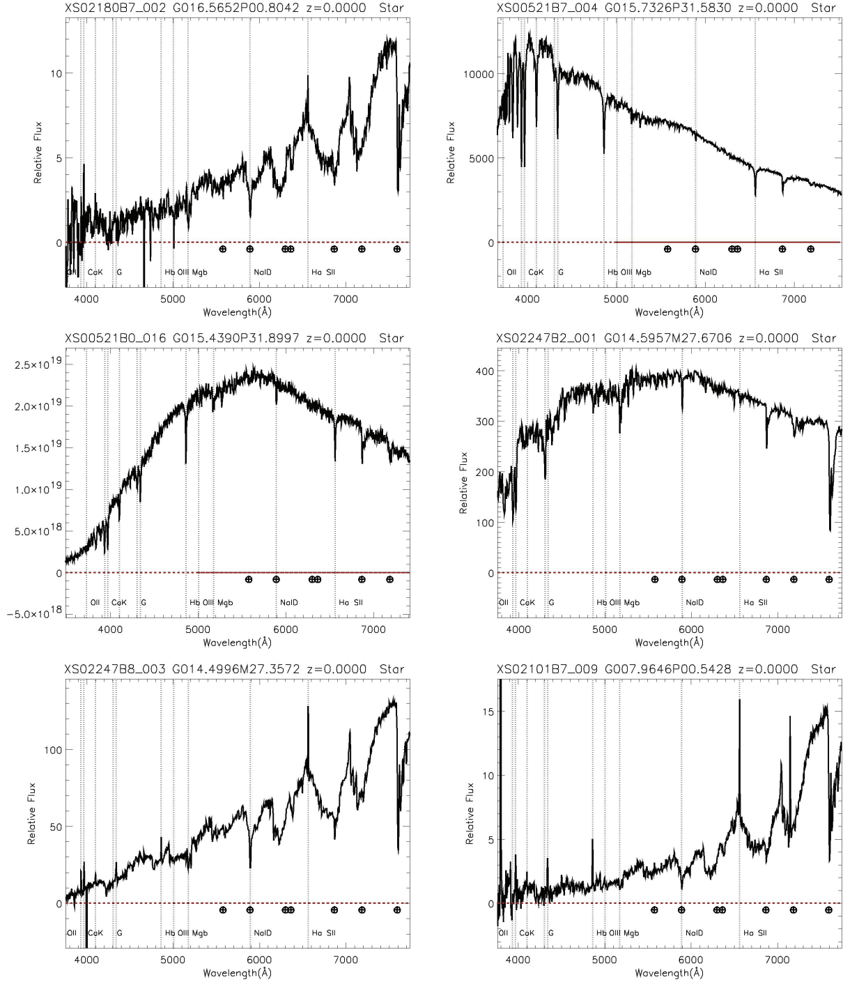
FIG. 3.— Example ChaMP spectra of stellar objects observed with FAST. CHANDRAOBSID, SPECOBJID, REDSHIFT and CLASS are given in the top of each plot.
