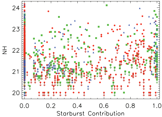
FIG. 13.— Percentage of starburst contribution to the bolometric luminosity versus column density in logarithmic scale. Downward arrows represent the 90% upper limits to N_H^{intr} , whenever the 90% lower limit encompassed zero. Red circles, green squares and blue triangles denote broad-line AGN, narrow emission line and absorption line galaxies respectively.
