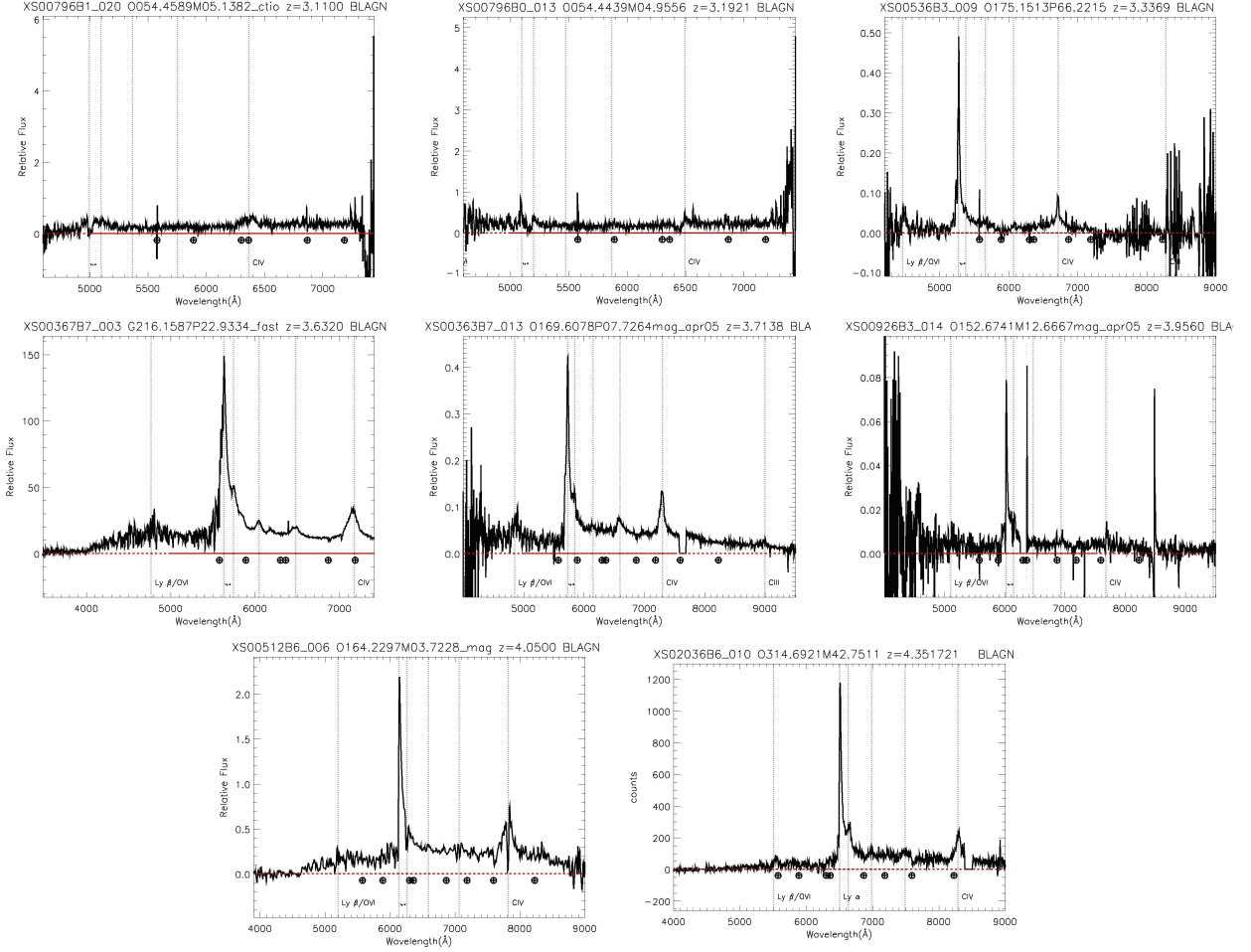
FIG. 15.— ChaMP z > 3 objects obtained using CTIO, FAST, WIYN and Magellan telescopes. Spectra are not flux calibrated. CHANDRAOBSID, SPECOBJID, REDSHIFT and CLASS are given in the top of each plot.
