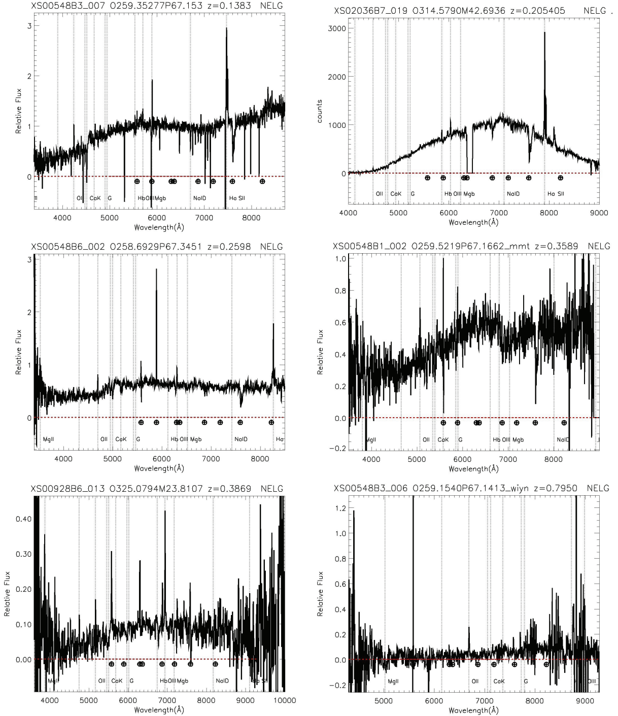
FIG. 5.— Example ChaMP spectra of narrow emission line galaxies observed with Magellan, MMT and WIYN telescopes. Spectra are not flux calibrated. CHANDRAOBSID, SPECJOBID, REDSHIFT and CLASS are given in the top of each plot.
