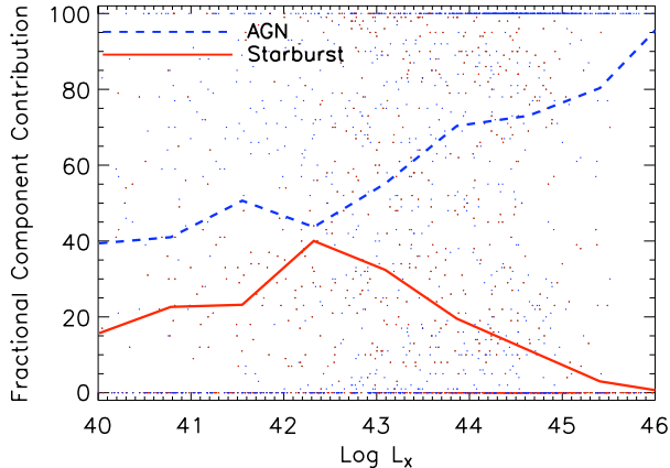
FIG. 11.— Fractional contribution of AGN (blue dots) and starburst components (red dots) to bolometric luminosity versus \log L_X . Points represent the fractional AGN and/or starburst contributions for all objects with L_{X(2-10keV)} > 10^{40} erg s ^{-1} . Solid red line represents the average value of starburst fractional contribution per \log L_X bin of 0.6. Dashed blue line represents the average value of AGN fractional contribution per \log L_X bin of 0.6.
