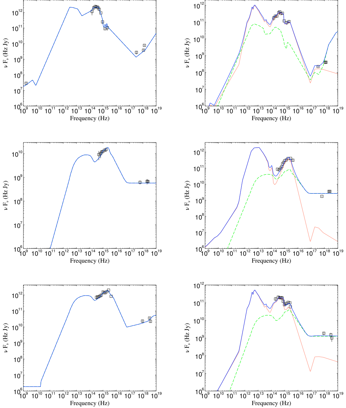
FIG. 8.— Examples of best-fit SEDs (blue line). Red solid and green dashed lines are the starburst and AGN templates respectively. Square boxes indicate available photometry. Vertical lines are associated >10\% errors. Top Left : XS0518B7007 with L_{2-10\text{ keV}}=1.1\times 10^{40}\text{ erg s}^{-1} at z = 0.08 . Best fitted with a Seyfert-2 NGC3393 template. Top Right : XS05618B6006 with L_{2-10\text{ keV}}=3.1\times 10^{40}\text{ erg s}^{-1} at z = 0.08 . Best fitted with a Seyfert-2 NGC4507 and a starburst NGC7714 templates, contributing 15% and 85% respectively to the L_{BOL} . Middle Left : XS00546B2012, with L_{2-10\text{ keV}}=9.1\times 10^{43}\text{ erg s}^{-1} at z = 1.01 . Best fitted with an Elvis et al QSO template. Middle Right : XS02251B7002, with L_{2-10\text{ keV}}=9.5\times 10^{43}\text{ erg s}^{-1} at z = 1.1 . Best fitted with an Elvis et al QSO and a starburst NGC5253 templates, contributing 15% and 85% respectively to the L_{BOL} . Bottom Left : XS0907B3001 with L_{2-10\text{ keV}}=9.6\times 10^{44}\text{ erg s}^{-1} at z = 2.08 . Best fitted with a Hopkins et al (2007) QSO template. Bottom Right : XS04151B6006 with L_{2-10\text{ keV}}=4.1\times 10^{44}\text{ erg s}^{-1} at z = 1.92 . Best fitted with a Hopkins et al. QSO and a starburst NGC7714 templates, contributing 20% and 80% respectively to the L_{BOL} .
