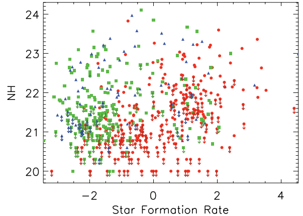
FIG. 12.— Star formation rates versus column density in logarithmic scale. Downward arrows represent the 90% upper limits to N_H^{intr} , whenever the 90% lower limit encompassed zero. Red circles, green squares and blue triangles denote broad-line AGN, narrow emission line and absorption line galaxies respectively.
