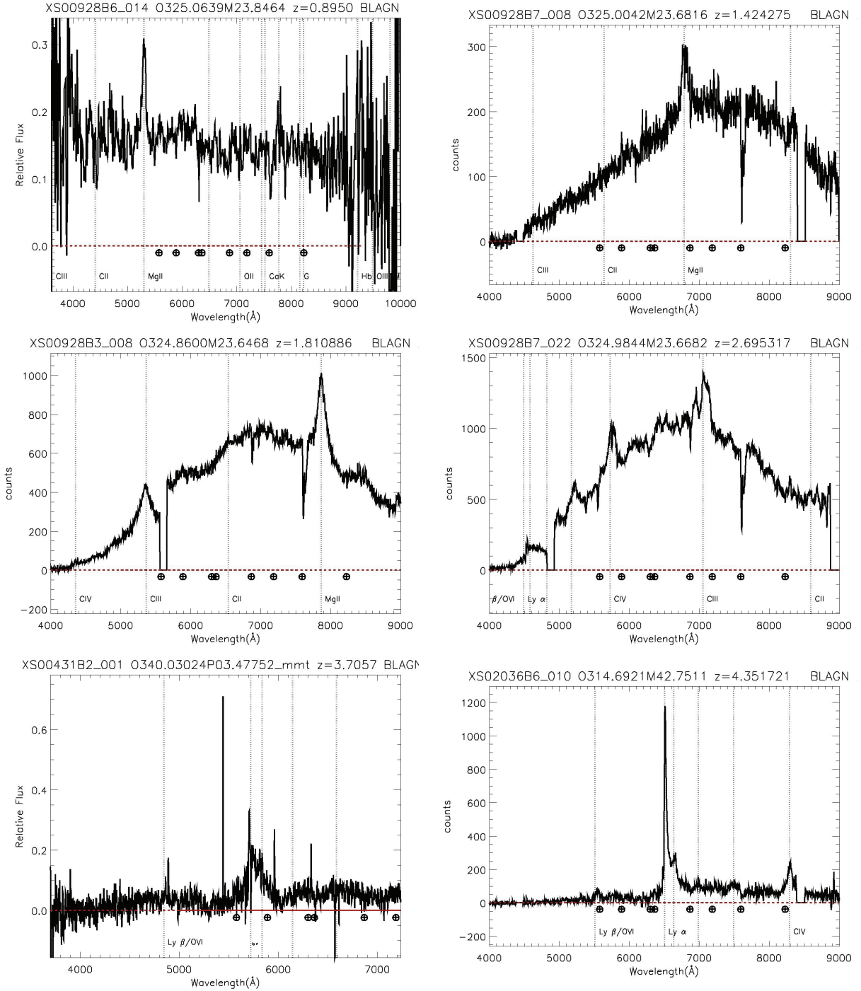
FIG. 6.— Example ChaMP spectra of broad line AGN observed with Magellan, MMT and WIYN telescopes. Spectra are not flux calibrated. CHANDRAOBSID, SPECJOBID, REDSHIFT and CLASS are given in the top of each plot.
