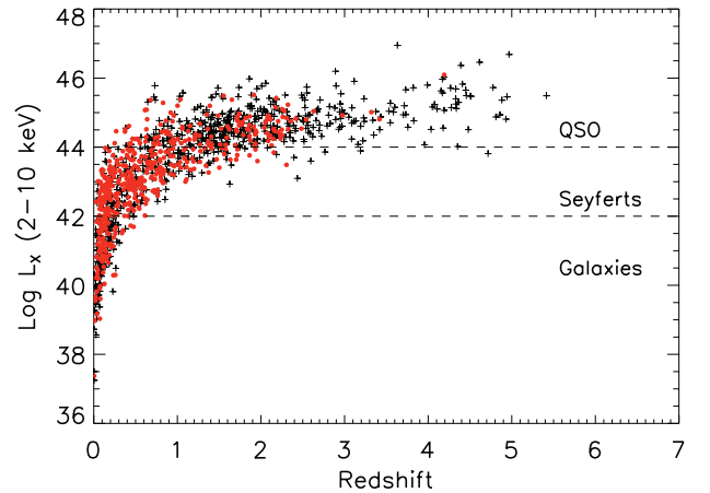
FIG. 10.— Distribution of rest-frame Logarithmic 2-10 keV X-ray luminosity and spectroscopic redshift for the 1202 hard-band X-ray detected sources from ChaMP. Red circles are sources that require a starburst component to fit available photometry. Black crosses are sources that their SED fits do not require any contribution from a starburst component. It is evident that as the X-ray luminosity increases, the occurrence of star formation activity decreases.
