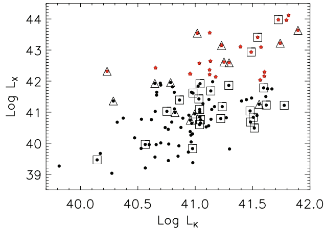
FIG. 14.— Rest-frame 2–10 keV logarithmic X-ray luminosity versus logarithmic K-band luminosity for all ChaMP spectroscopically identified absorption line galaxies with K-band detections. Red stars is the population of 25 XBONGs, ALGs with L_{X(2-10\text{ keV})} > 1.5 \times 10^{42} erg \text{s}^{-1} . Open triangles are radio loud sources. Open squares are sources with \log N_H^{\text{intr}} > 22 .
