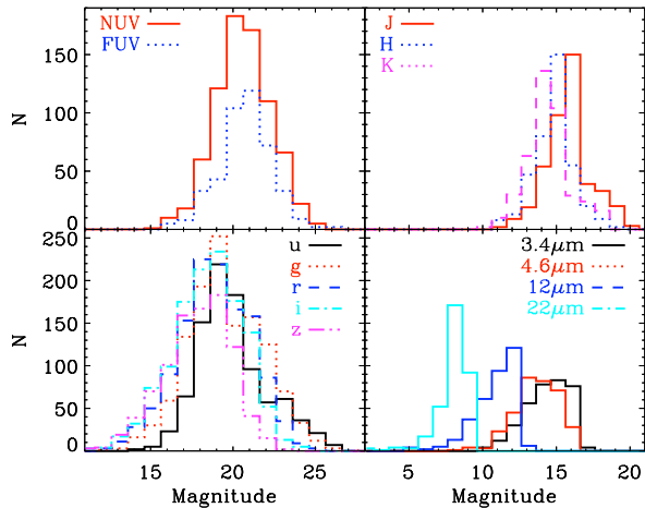
FIG. 2.— Multi-wavelength magnitude distributions for all our 1242 spectroscopically identified ChaMP extragalactic sources. UV and optical magnitudes are in the AB system, near- and mid-infrared magnitudes are in the Vega system.
