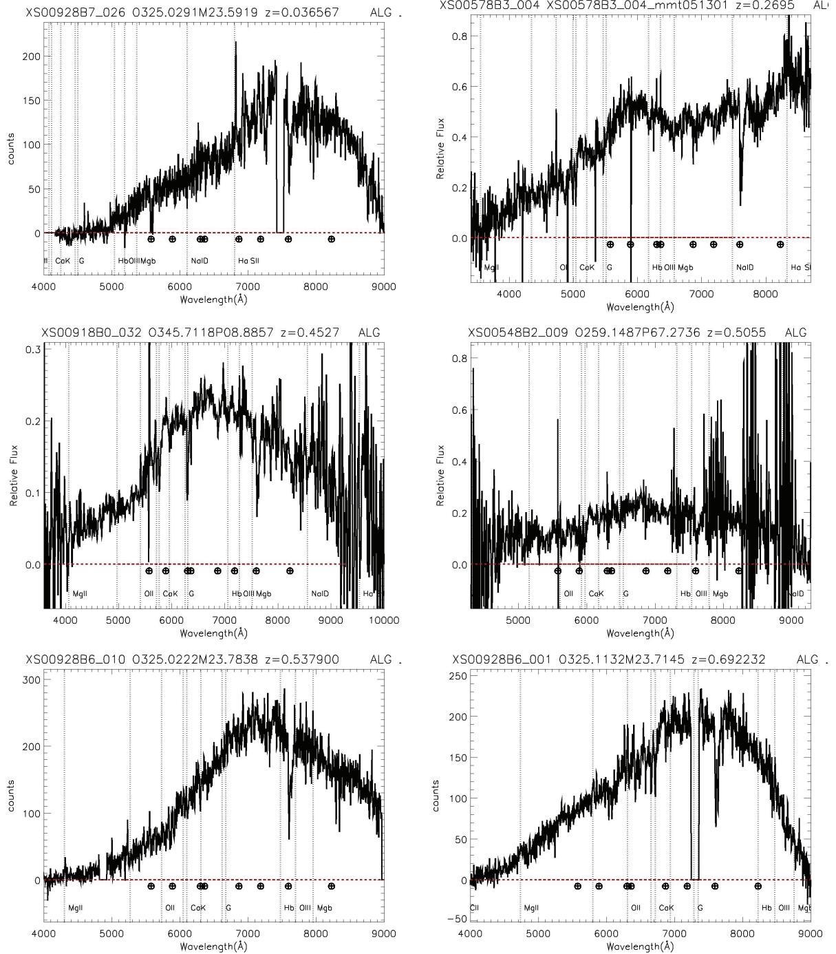
FIG. 4.— Example ChaMP spectra of absorption line galaxies observed with Magellan, MMT and WIYN telescopes. Spectra are not flux calibrated. CHANDRAOBSID, SPECJOBID, REDSHIFT and CLASS are given in the top of each plot.
