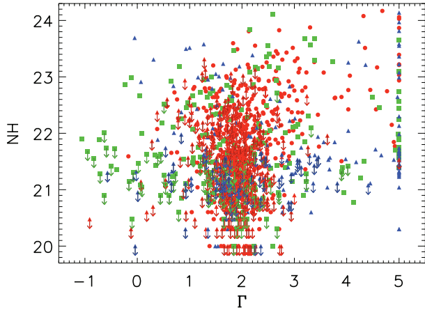
FIG. 9.— Best fit X-ray spectral slope \Gamma versus column density in logarithmic scale. Downward arrows represent the 90% upper limits to N_H^{intr} , whenever the 90% lower limit encompassed zero. Red circles, green squares and blue triangles denote broad-line AGN, narrow emission line and absorption line galaxies respectively.
