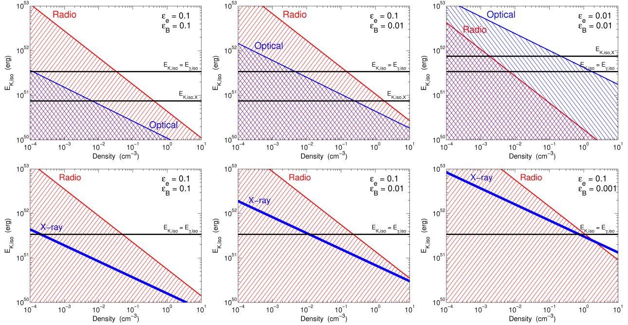
FIG. 9.— The phase-space of isotropic-equivalent blastwave kinetic energy and circumburst density delineated by the X-ray detection (thick line) and the optical and/or radio upper limits (hatched regions). The top row is for the case \nu_c < \nu_X , with the X-ray detection providing a measure of the E_{K,iso} (horizontal line). The bottom row is for the case \nu_c > \nu_X for which the optical limit is redundant with respect to the X-ray detection. Here the case of E_{K,iso} = E_{\gamma,iso} is marked by the horizontal black line. The panels are for different combinations of \epsilon_e and \epsilon_B .
