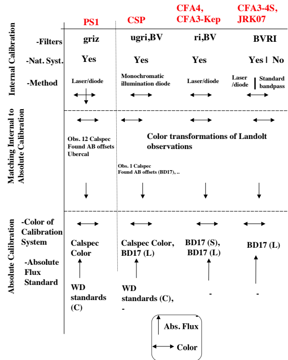
FIG. 1.— A schematic of the calibration of the PS1+lz sample. The calibration of the various subsamples is broken into three parts: ‘Internal calibration’ (filter measurements), ‘match between Internal and Absolute calibration’, and ‘Absolute calibration’. Arrows show whether in each step there may be an uncertainty due to a color measurement or absolute flux measurement. Directionality of absolute flux arrows show the source of the uncertainty. ‘C’, ‘L’ and ‘S’ represent the HST Calspec, Landolt and Smith standards respectively.
