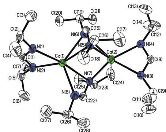
Figure 1. Solid-state structure of 1 with the thermal ellipsoids set at the 30% probability level; hydrogen atoms and the minor positions (15%) of the disordered bridging ligands are omitted for clarity. Selected distances [Å]: Ca(1)–N(1) 2.347(3), Ca(1)–N(5) 2.633(3), Ca(1)–N(7) 2.619(3), Ca(1)–N(8) 2.407(4), Ca(2)–C(24) 3.102(6). [27]
