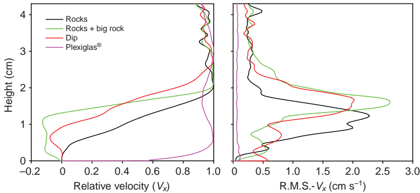
Fig. 6. Height and variability of the Plexiglas ® and rock-associated boundary layers and other regions of reduced flow resulting from water movement over each of four substrate types: Plexiglas ® , rocks, dip and rocks + big rock. (A) Profiles of relative velocity ( x -direction) versus height above the four substrates. Velocity data for each substrate type are scaled to a value of 1.0 to account for differences in the free-stream flow speed at which video sequence data were collected. (B) r.m.s.- V_x profiles versus height above the top of the same four substrates. Both velocity and r.m.s.- V_x values were calculated from sequences of 1000 (Plexiglas ® ), 400 (rocks and dip) or 600 (rocks + big rock) frames. Note that the same sequences also appear in Figs 2–5.
