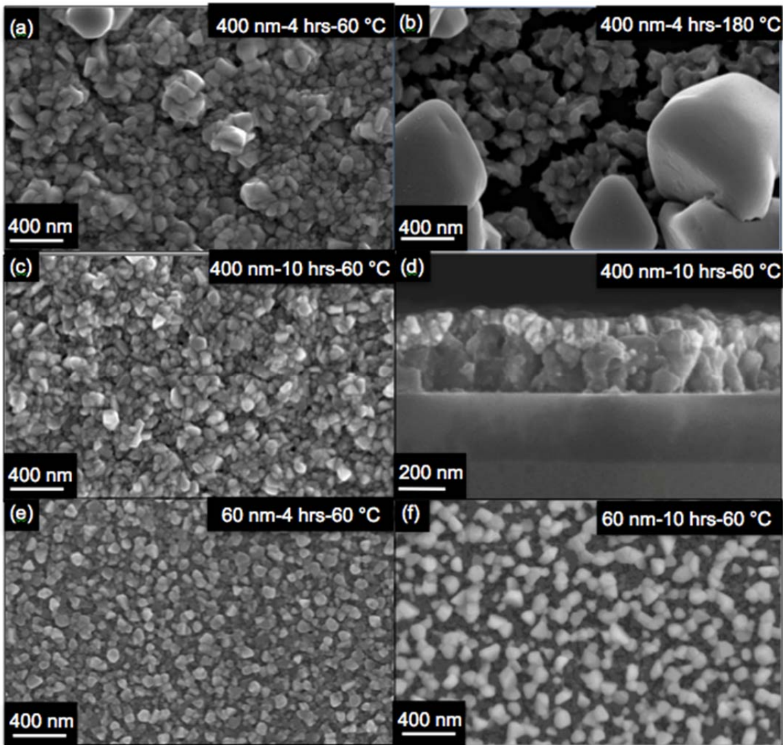
FIG. 4. SEM images of Cu 2 S films with initial thickness x , exposed to HBr for y hours at a temperature of z °C (denoted x - y - z ) (a) 400 nm-4 hrs-60 °C; (b) 400 nm-4 hrs-180 °C; (c) 400 nm-10 hrs-60 °C; (d) 400 nm-10 hrs-60 °C imaged in cross-section; (e) 60 nm-4 hrs-60 °C; (f) 60 nm-10 hrs-60 °C.
