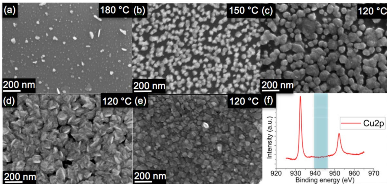
FIG. 1. (Color online) SEM images of \text{Cu}_2\text{S} film coverage after 322 cycles at a growth temperature of (a) 180 °C, (b) 150 °C, and (c) 120 °C. 120 °C was selected for its superior film coverage and \text{Cu}_2\text{S} films were deposited for (d) 400 and (e) 500 cycles. A high-resolution XPS scan of the \text{Cu}2p region shown in (f) gives no indication of the \text{Cu}^{2+} satellite peak typically observed at 943 eV (highlighted region).
