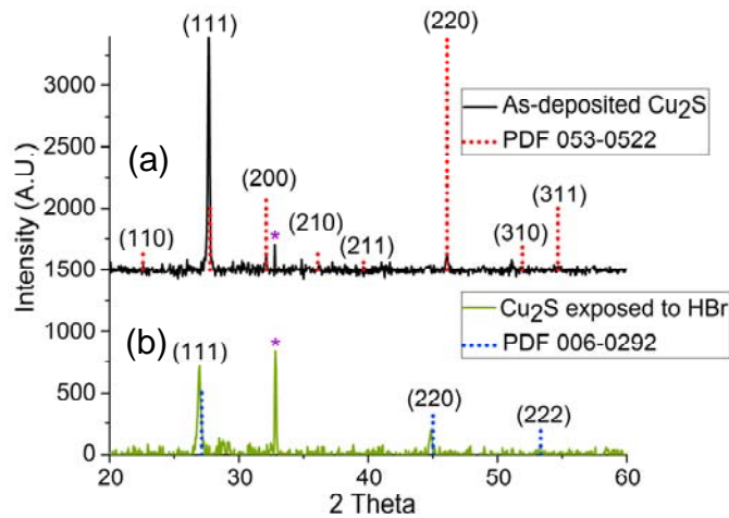
FIG. 3. (Color online) X-ray diffraction patterns of as-deposited 250 nm thick \text{Cu}_2\text{S} film (top) and the same film after conversion of the top 100 nm to CuBr via a 4-hour exposure to HBr at 60 °C (bottom). The asterisk (*) denotes a background peak associated with the XRD instrument itself.
