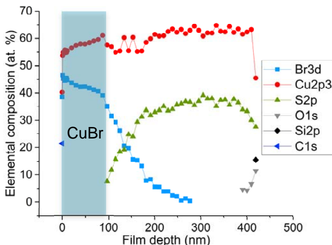
FIG. 2. (Color online) Depth profile obtained by XPS of a film converted from a 400-nm thick film of Cu 2 S.
