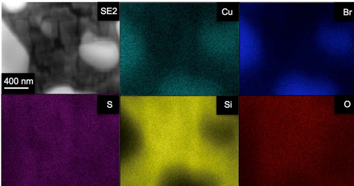
FIG. 5. (Color online) EDS composition mapping of a 400-nm thick film of \text{Cu}_2\text{S} exposed to HBr for 4 hours at 180 °C.
