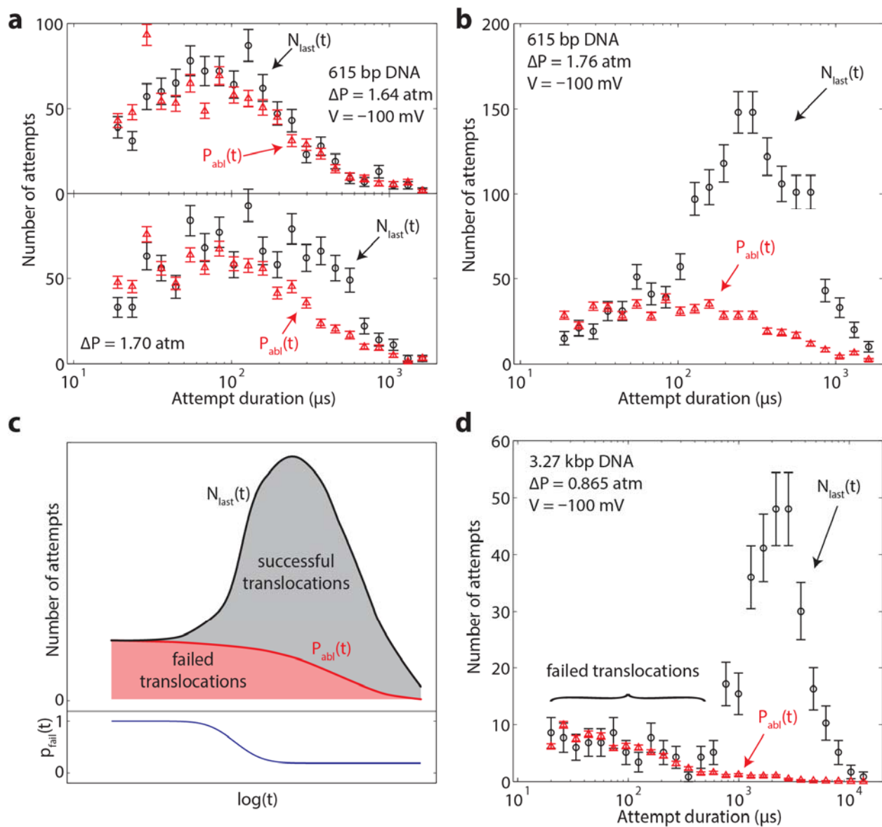
Figure 3. Analysis of failed translocations. (a-b) Logarithmic event duration histogram for 615 bp DNA at \Delta P = 1.64, 1.70, and 1.76 atm. (c) Upper panel is the schematic interpretations of the event duration histograms. Lower panel is the calculation of p_{\text{fail}}(t) used in the calculation of average trapped time of successful events. (d) Logarithmic event duration histogram for 3.27 kbp
