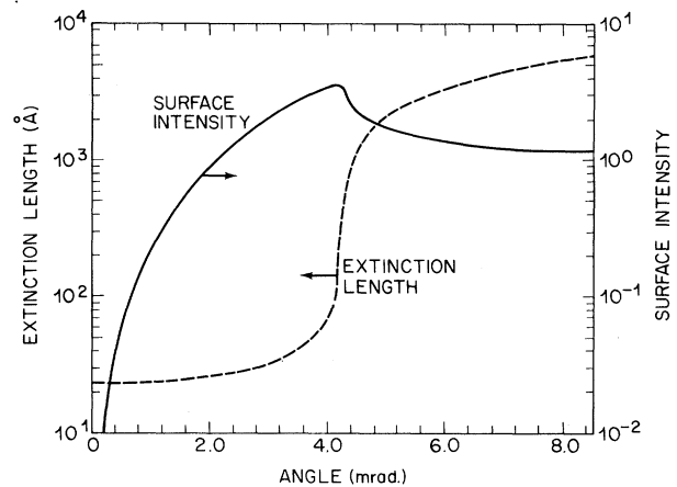
FIG. 3. Angular variation of penetration depth and surface intensity appropriate for the case of germanium.
