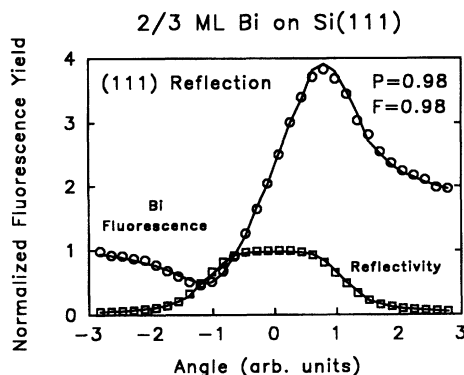
FIG. 1. The [111] reflectivity and fluorescence yield for \frac{2}{3} -ML Bi on \text{Si}(111) \sqrt{3} \times \sqrt{3} R30^\circ .
