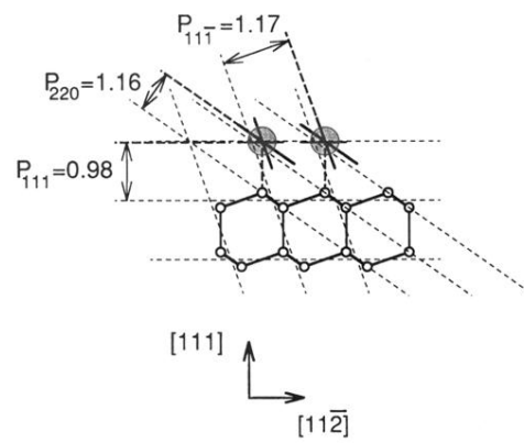
FIG. 3. The registration of the Bi atoms relative to the Si [111], [1\bar{1}\bar{1}] , and [220] planes.
