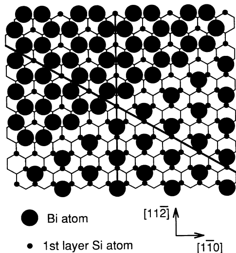
FIG. 5. An exact atomic model for the two phases shown in Fig. 4.
