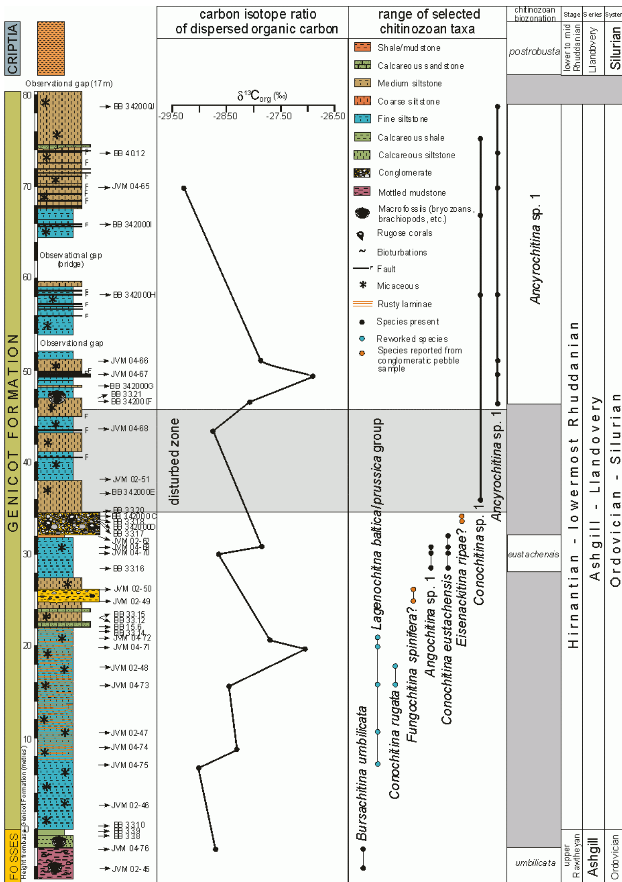
Figure 1: δ 13 C org isotope curve and chitinozoan distribution in the Parc de Sart-Eustache section. Chitinozoan biozonation and age assignment are figured on the right.
