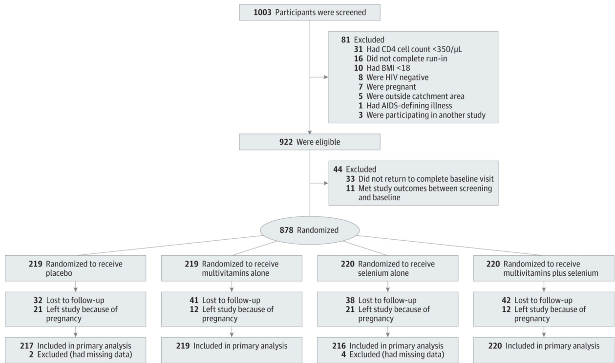
Figure 1. Randomization Flowchart
