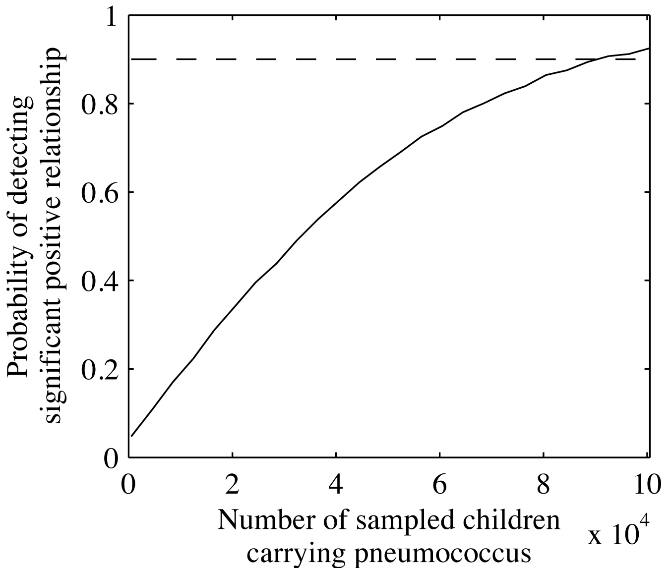
Figure 2. Probability of detecting a significant positive trend between serotype rank and the rate of co-colonization with H. influenzae for different sample sizes when H. influenzae significantly increases pneumococcal diversity ( c = 0.2 , H. influenzae prevalence = 25%, \sigma = 0.1 ). Serotypes are ranked in descending order of their frequency (or intrinsic duration of carriage), with rank 1 denoting the most common serotype and 25 the rarest. The sample size refers to the number of children <5 y old colonized with pneumococcus. The dashed line shows a 90% probability of detecting a significant positive trend by logistic regression.
