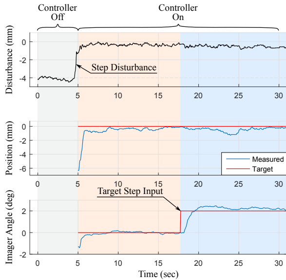
Fig. 11. Bench top tests demonstrating the ability of the robotic system to maintain the catheter tip at the target pose despite disturbance step and target step inputs.
