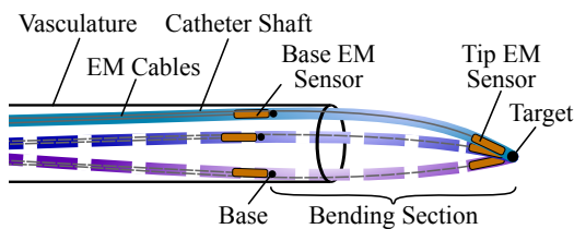
Fig. 3. Uncontrollable catheter shaft motion. Dashed lines show alternative locations of the catheter shaft due to uncontrolled motion within the vasculature. EM trackers measure the position and orientation of the catheter at two locations: at the base of the bending section, and at the tip.
