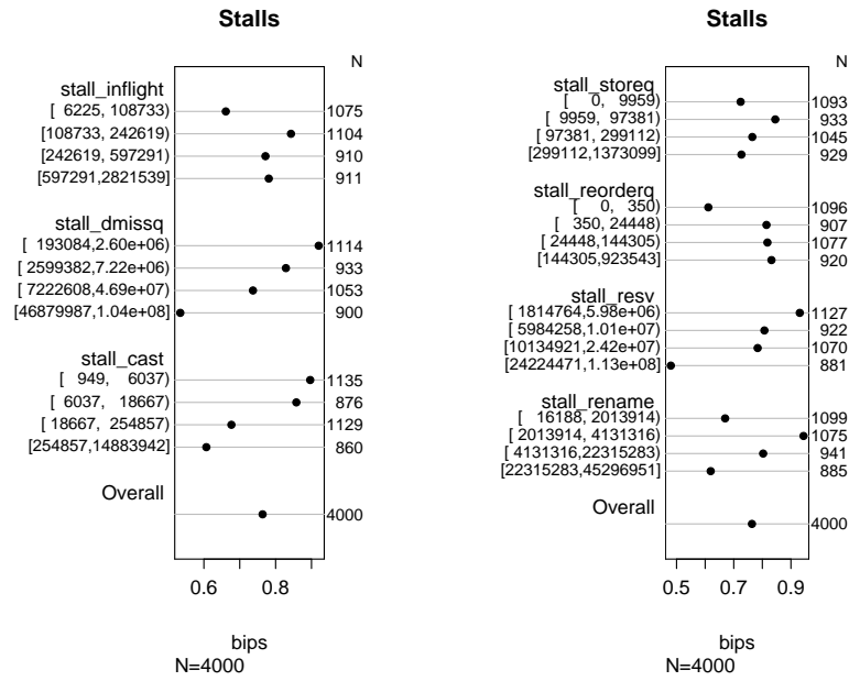
Figure 4: Association Plots. Application baseline stall behavior.
