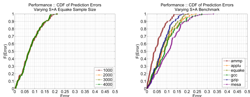
Figure 11: S+A Performance Model Sensitivity: Varying n_{S+A} (L) and benchmark (R).
