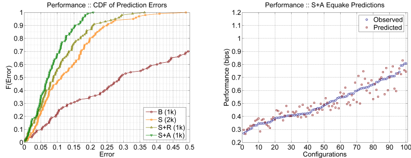
Figure 9: Empirical CDF of prediction errors with error minimizing sample and region sizes. Equake achieves median accuracy and is plotted for S+A (L). Prediction results for S+A (R).
