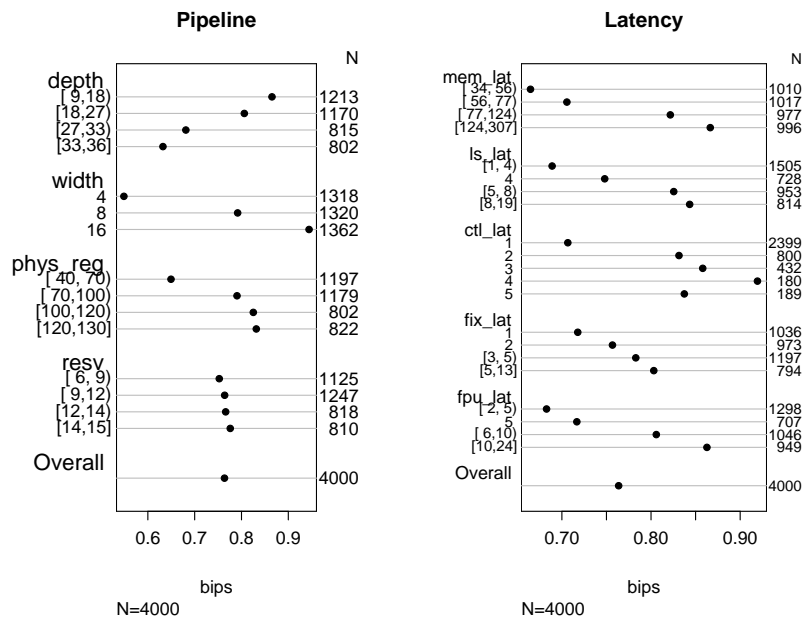
Figure 2: Association Plots. Measures of pipeline dimensions (L) and unscaled latencies (R).
