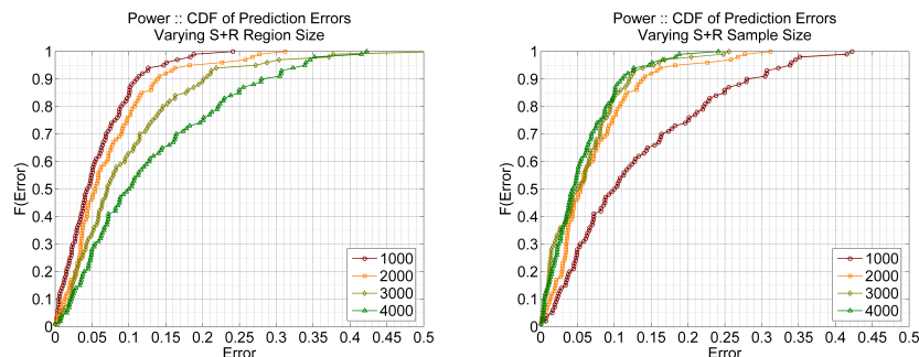
Figure 13: S+R Power Model Sensitivity: Varying r_{S+R} with fixed n_{S+R} = 4,000(L) and n_{S+R} with fixed r_{S+R} = 1,000 (R) .
