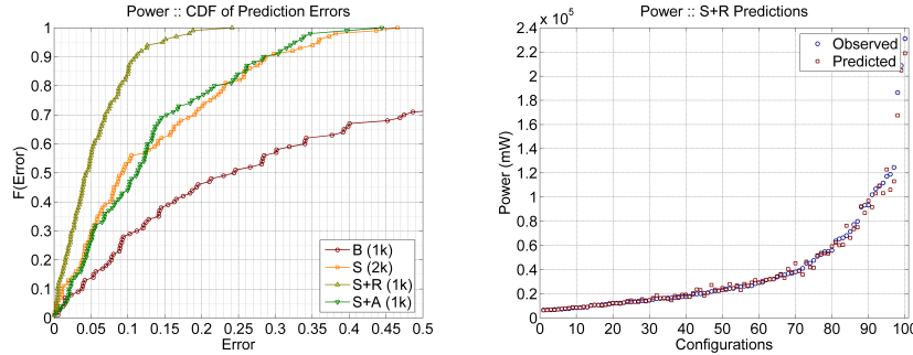
Figure 12: Empirical CDF of prediction errors with error minimizing sample and region sizes (L). Prediction results for S+R (R).
