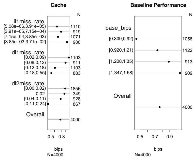
Figure 5: Association Plots. Application cache behavior (L) and baseline performance (R).
