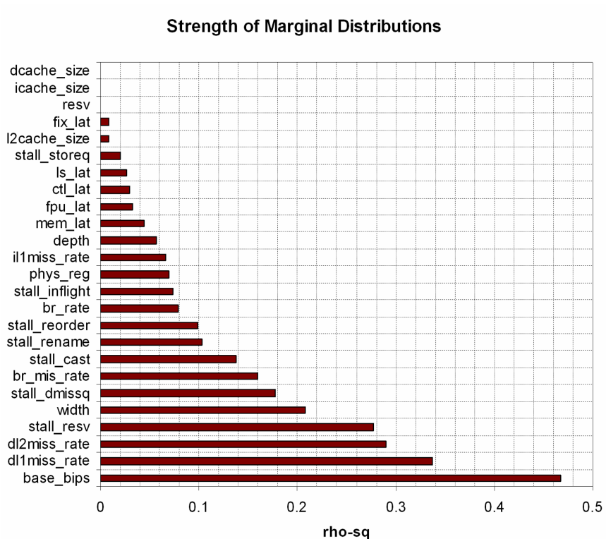
Figure 6: Strength of Marginal Relationships. A lack of fit for predictors with high \rho^2 will more consequentially impact performance prediction.
