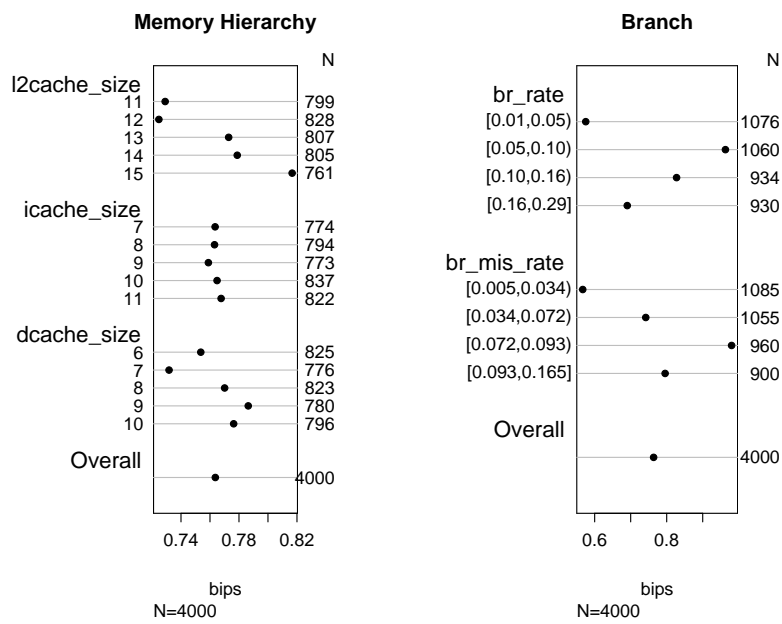
Figure 3: Association Plots. Memory hierarchy (L) and application branching behavior(R).
