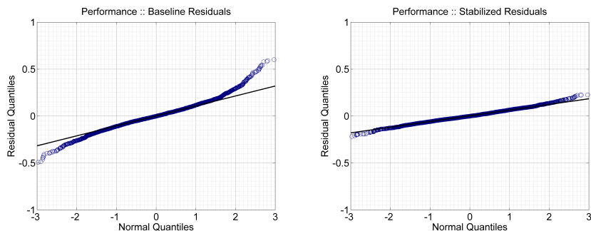
Figure 8: Quantile-Quantile Plots. Quantiles of residuals (y-axis) plotted against normal quantiles (x-axis). A line is drawn between the second and third quartile of the residuals to check linearity.
