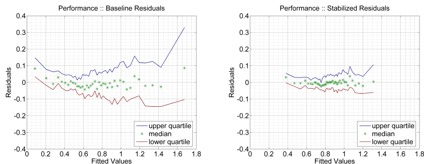
Figure 7: Residual Plots. Quartiles of residuals, stratifying 4000 fitted performance into groups of 100, before (L) and after(R) variance stabilization. The x-coordinate is the mean predicted performance of the 100 group members.
