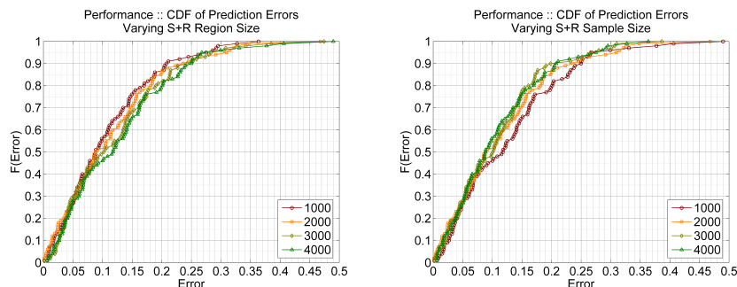
Figure 10: S+R Performance Model Sensitivity: Varying r_{S+R} with fixed n_{S+R} = 4,000 (L) and n_{S+R} with fixed r_{S+R} = 1,000 (R).
