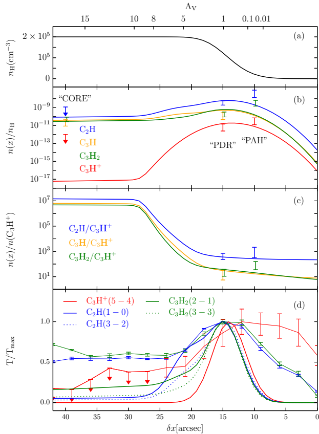
FIG. 3.— Photochemical model of the Horsehead PDR. (a) Density profile n_{\text{H}} = n(\text{H}) + 2n(\text{H}_2) . (b) Predicted abundance of small hydrocarbons. (c) Predicted abundance ratio relative to l\text{-C}_3\text{H}^+ . (d) Predicted intensity profile. Two lines are included for \text{C}_2\text{H} : N = 1 - 0 ( E_u/k \sim 4 K) and N = 3 - 2 ( E_u/k \sim 25 K); and for c\text{-C}_3\text{H}_2 : J = 2 - 1 ( E_u/k \sim 6 K) and J = 3 - 2 ( E_u/k \sim 16 K). The observed intensity profile is overlaid with error bars.
