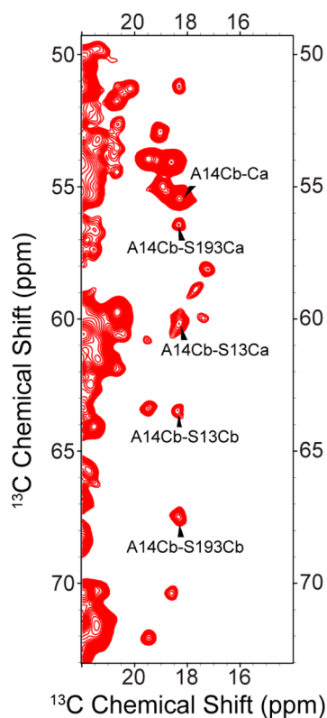
Figure 4. Expansion of the PAR spectrum of Figure 3. Long mixing ^{13}\text{C} – ^{13}\text{C} experiment on [\text{U-}^{13}\text{C},^{12}\text{C}\text{-WHIFY},^{15}\text{N}] VDAC obtained with 14 ms CC PAR. Selected assignments are shown for A14–S13 and A14–S193 contacts.
