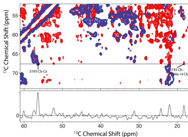
Figure 3. Fourteen millisecond ^{13}\text{C} – ^{13}\text{C} PAR (red) of [\text{U-}^{13}\text{C},^{12}\text{C}\text{-WHIFY},^{15}\text{N}] VDAC overlaid on a 1.8 ms RFDR (blue) spectrum of [\text{U-}^{13}\text{C},^{15}\text{N}] VDAC showing the unambiguous contact between S193 Cb and A14 Cb. Both spectra were acquired at \omega_{\text{OH}}/2\pi = 900 MHz and \omega_r/2\pi = 20 kHz.
