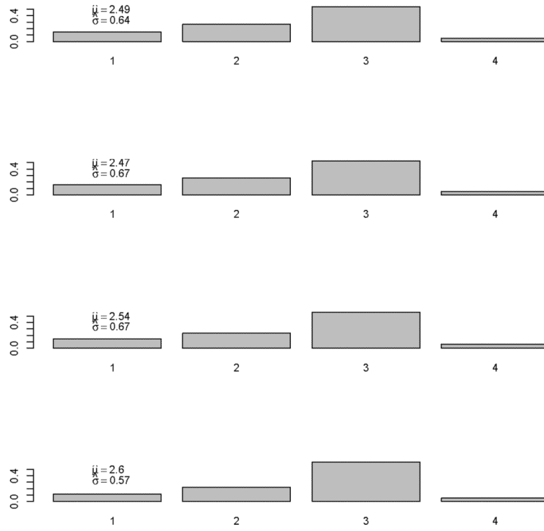
Figure 5. Serial interval estimate using data up to and including 4/25/2009 (top figure), 4/26/2009 (second), 4/27/2009 (third) and 4/28/2009 (bottom figure).
