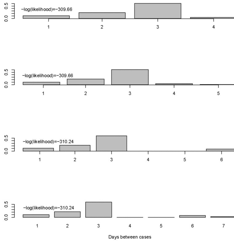
Figure 3. Serial interval estimates for k=4, 5, 6, and 7 days with -\log(\text{likelihood}) values.
