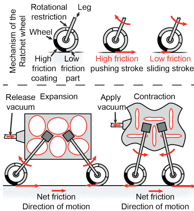
b) Schematic of buckling walker
