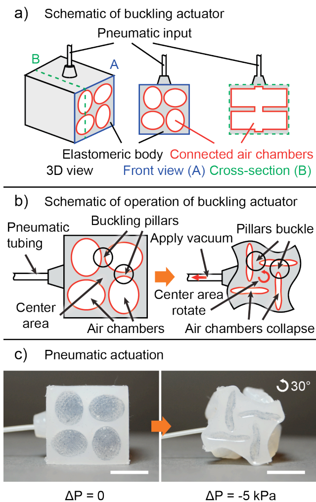
Figure 1. Schematics of a single-unit buckling actuator. a) A buckling actuator unit consists of an elastomeric structure with a non-buckling center area connecting to several buckling pillars, with air chambers in between. The air chambers are actuated externally through a single pneumatic input. b) The rotary actuation mechanism of buckling actuator. Vacuum induces overall compression of the structure, causing the buckling pillars to deform into predetermined shapes. The cooperative deformation causes the center area to rotate in one preferred direction. c) Images of a single-unit buckling actuator in the initial
