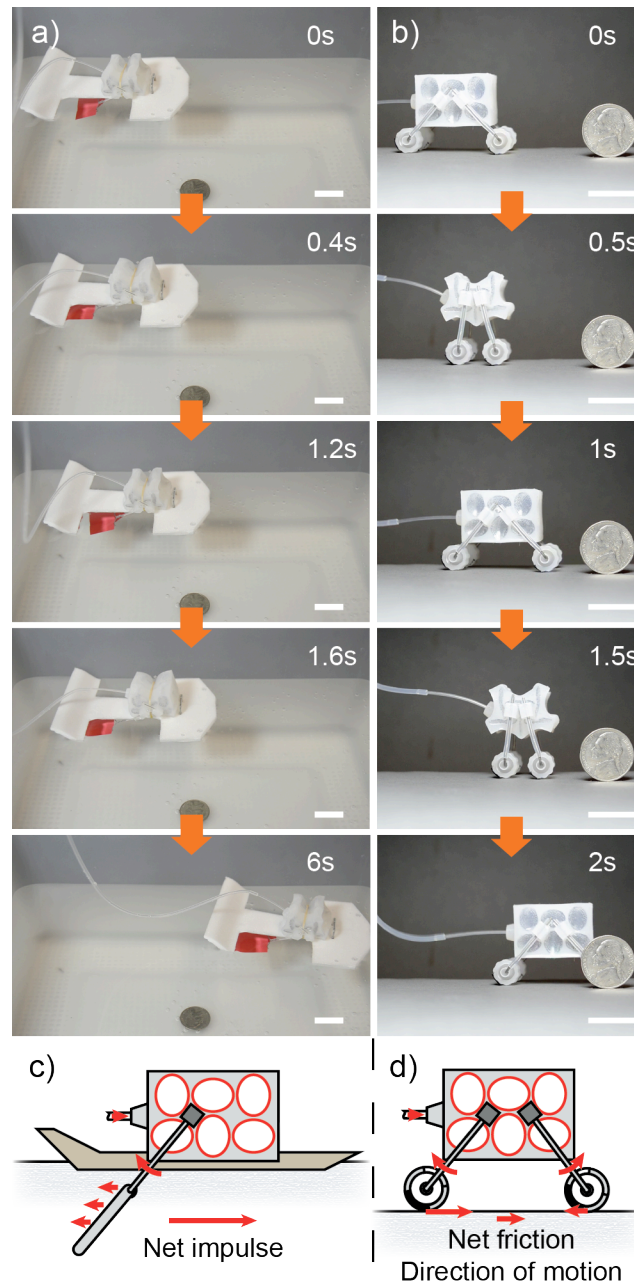
Figure 4. Soft robots with buckling actuators. a) A soft robotic swimmer. b) A soft robotic walker. c) Schematics of the swimmer. d) Schematics of the walker. Scale bars are 2 cm. The SI illustrates the motion of the cart in greater detail.
