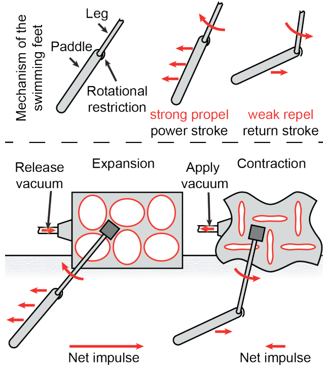
a) Schematic of buckling swimmer
