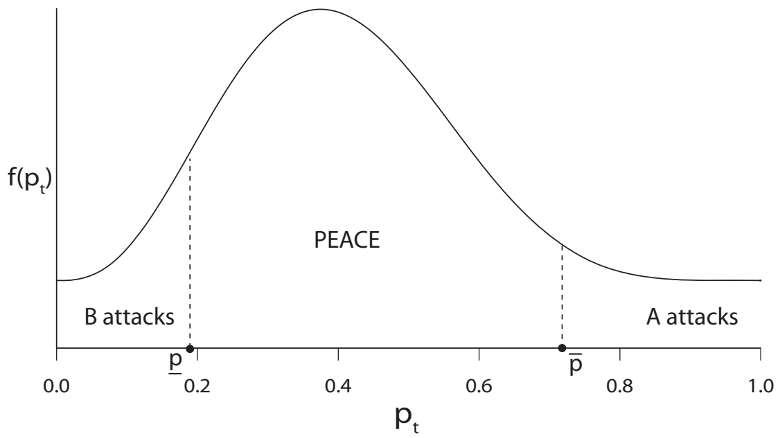
Figure 2: States' Equilibrium Cutpoints in the Recurring Diffusion Model
