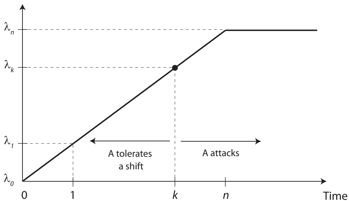
Figure 1: Gradually Increasing \lambda_t and Delayed Attack
