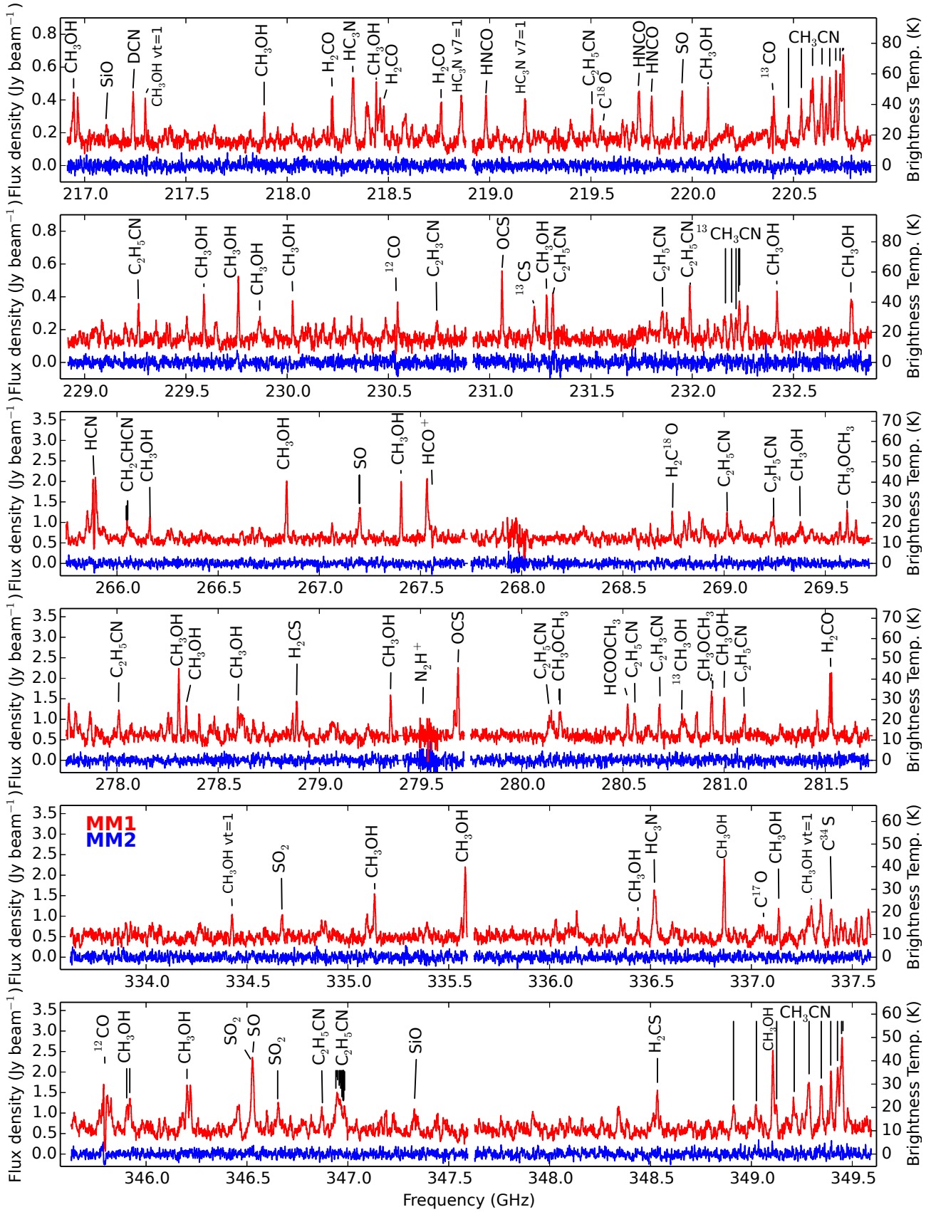
Fig. 2.— Continuum-subtracted SMA spectra towards the MM1 (red) and MM2 (blue) continuum peaks, showing the full 24 GHz SMA bandwidth. MM1 spectra are offset for clarity. Transition frequencies for selected molecules are labeled for reference.
