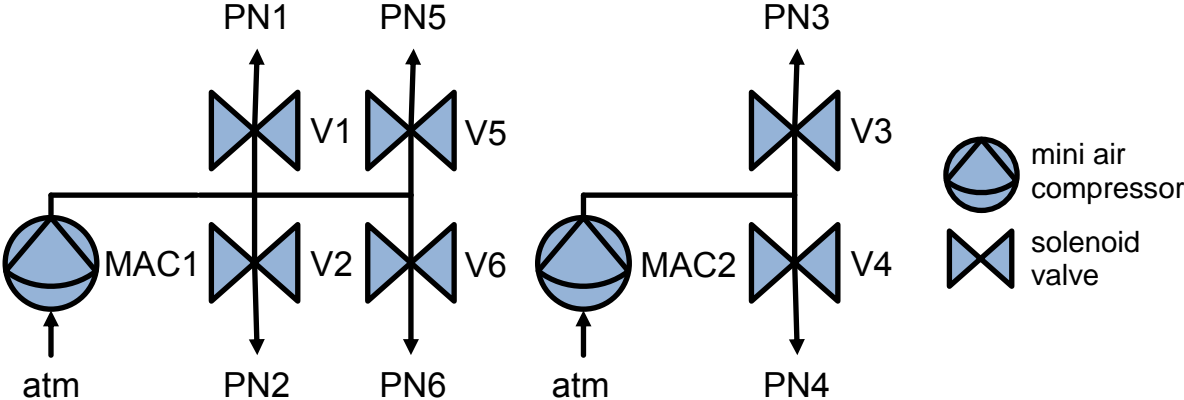
Figure S1. Systems diagram of the configuration of mini air compressors and valves used to drive the robot in undulation or walking gaits.
