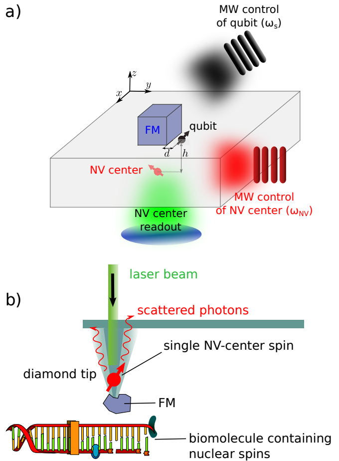
Figure 1. Panel a) shows a detailed illustration of the setup considered. The abbreviation “FM” denotes the ferromagnetic particle that is placed on top of the diamond surface that contains the NV-center (red) which is used as magnetometer. Close to the top surface of the FM lies the qubit (black) we want to measure. The setup also includes separate microwave (MW) controls of the qubit (black) and NV-center (red) with resonance frequencies \omega_s and \omega_{NV} , respectively. The ferromagnetic resonance frequency \omega_F is assumed to be different from both \omega_s and \omega_{NV} . The NV-center is read out optically with a green laser. A slightly modified version of the setup with the NV-center and the FM on a tip is illustrated in panel b); for simplicity we have omitted the two driving fields in this panel.
