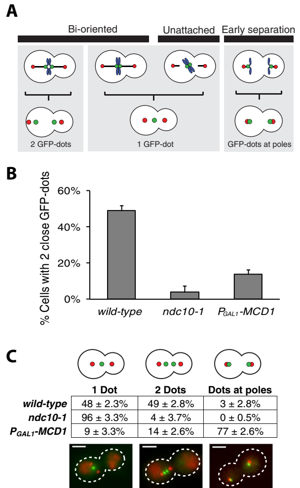
FIGURE 3: Confirming kinetochore and cohesin inactivation. (A) Chromosome attachment schematic. Correct attachment of a chromosome to the spindle results in biorientation, visualized as two GFP dots separated by \leq 1 \mu\text{m} . A single GFP dot is a kinetochore pair separated by < 0.3 \mu\text{m} or a chromosome attached to only one or neither spindle pole (red dots). Cohesin-less chromosomes separate prematurely during metaphase. GFP dots at poles are separated by > 1 \mu\text{m} . (B) Chromosome biorientation. ndc10-1 and P_{GAL1} - MCD1 strains have few bioriented chromosomes compared with wild type. Error bars are SDs. (C) Chromosome position. Positions of GFP dots were scored to distinguish between unattached (one dot, ndc10-1 ) and prematurely separated sister chromatids (two dots, P_{GAL1} - MCD1 ). Error bars are SDs. Scale bar, 3 \mu\text{m} .
