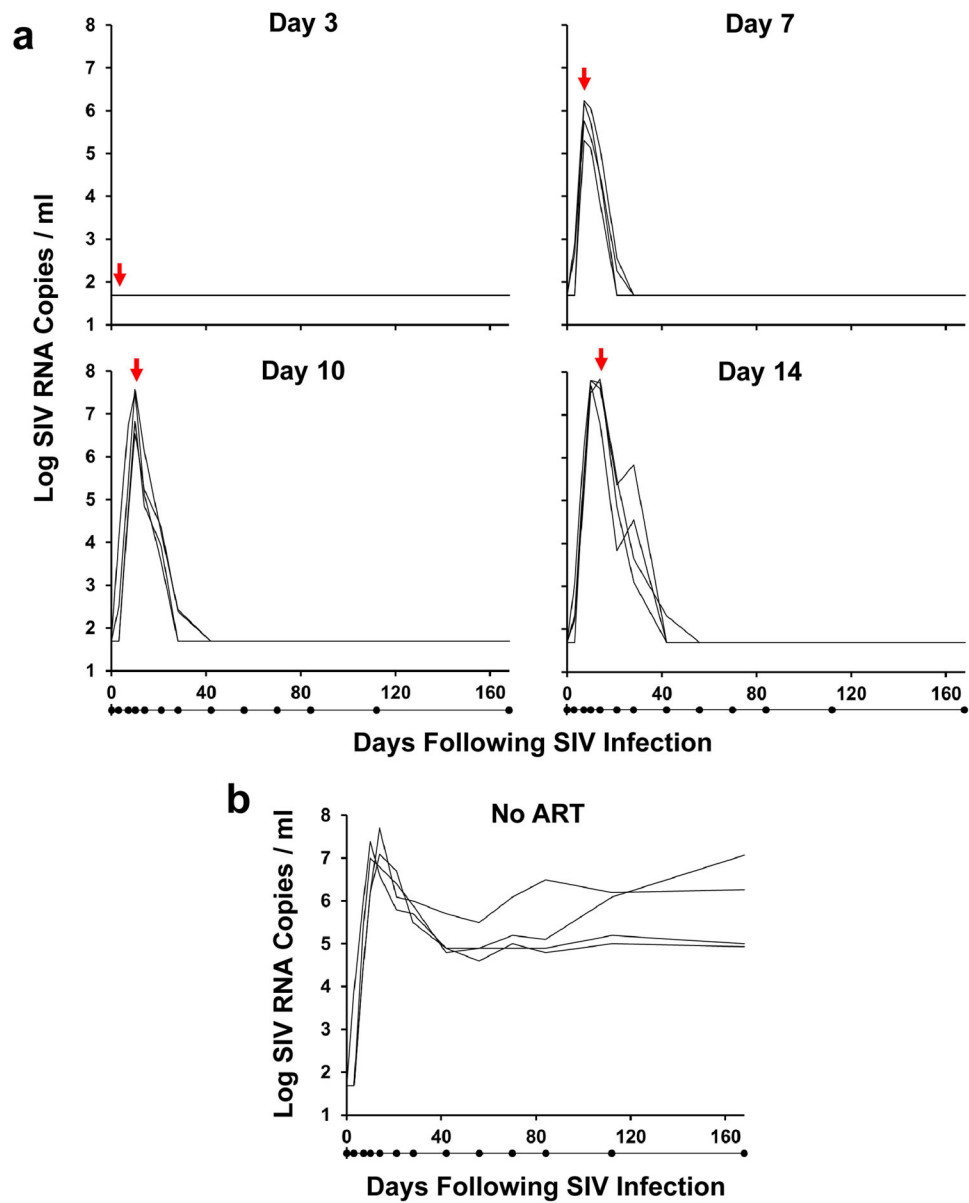
Figure 1. Viral decay kinetics after treatment with ART Log plasma viral RNA (copies/ml) in rhesus monkeys infected with SIVmac251 and following initiation of ART on days 3, 7, 10, and 14 of infection ( a ) or with no ART ( b ). Assay sensitivity is 50 RNA copies/ml. Red arrows indicate initiation of ART. Black dots below x-axis indicate sampling timepoints.
