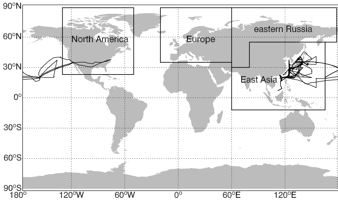
Figure 1. Tagged source regions for the CH 4 , C 2 H 6 , and CO simulations. “Eurasia” in the text refers to the combination of Europe and eastern Russia. The TRACE-P flight tracks are also shown.
