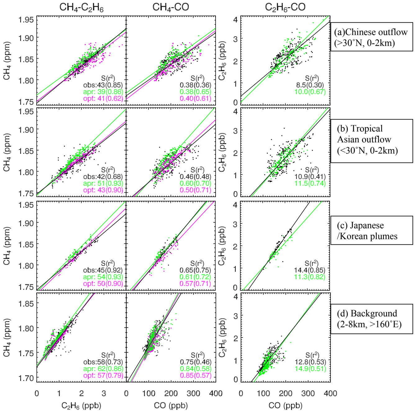
Figure 6. Simulated vs. observed CH 4 -C 2 H 6 -CO correlations along the TRACE-P flight tracks in different regions. (a) Chinese outflow (>30°N and <2km, west of 160°E); (b) tropical Asian outflow (<30°N and <2km, west of 160°E); (c) Japanese/Korean plumes; (d) background (2-8km, east of 160°E). TRACE-P observations (“obs”, black) are compared to a priori model results (“apr”, green) and optimized model results (“opt”, red). The slopes (S) and r^2 of the RMA regression lines are shown (also in Table 3).
