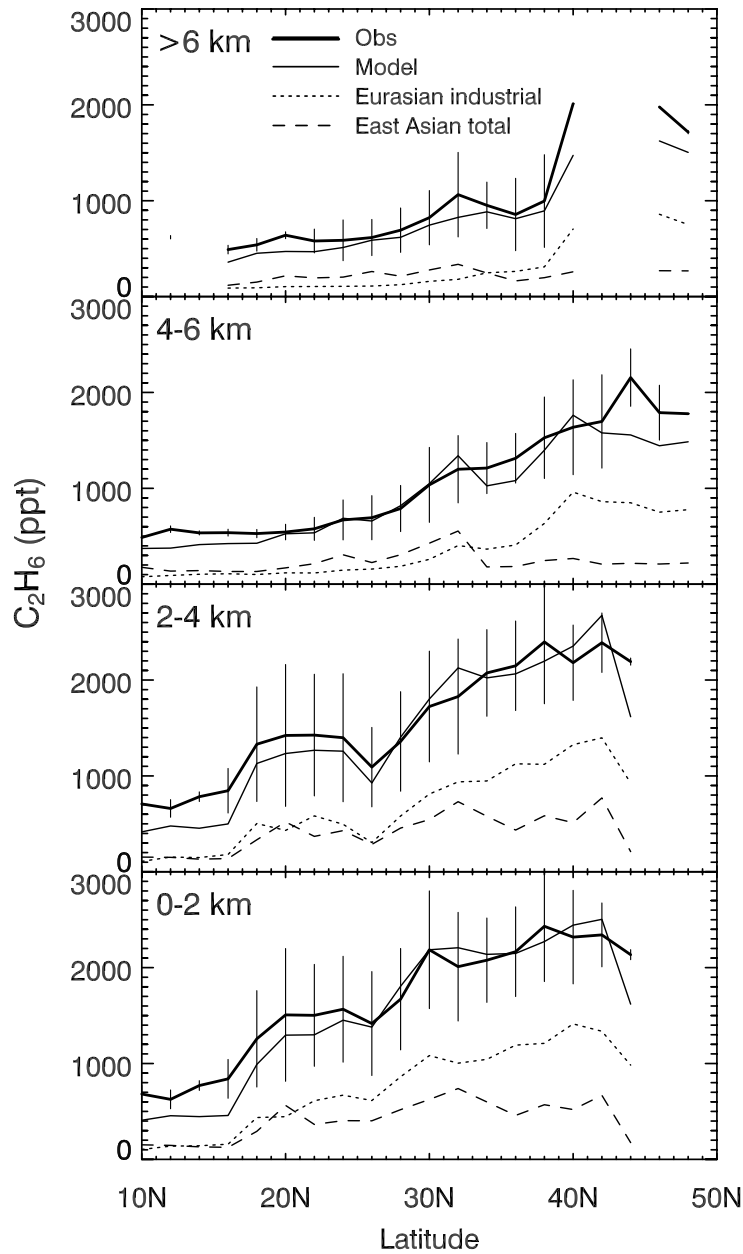
Figure 5c. Latitudinal dependence of C 2 H 6 concentrations along the TRACE-P flight tracks west of 160°E during TRACE-P at different altitudes. Observations (thick lines) are compared to model results (solid lines). The error bars represent standard deviations for the observations. Contributions of C 2 H 6 from East Asian (dashed) and Eurasian (dotted) tagged tracers in the model are also shown.
