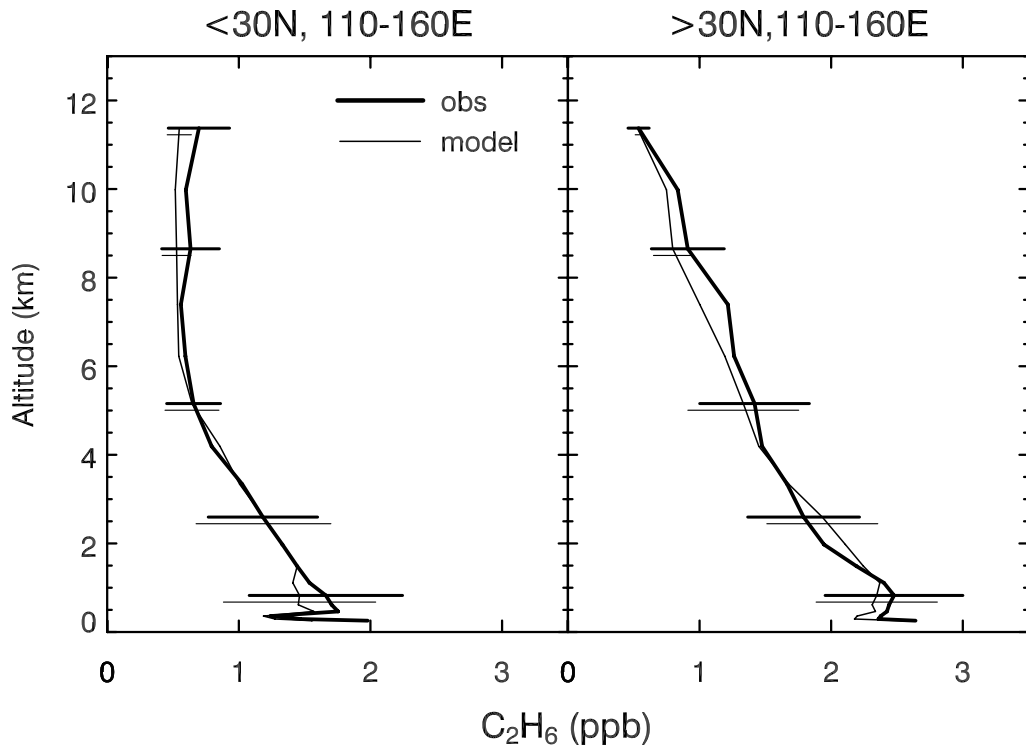
Figure 5b. Mean vertical profiles of C_2H_6 concentrations along the TRACE-P flight tracks, north of 30^\circ N and south of 30^\circ N at 110^\circ E - 160^\circ E (NW Pacific, Asian outflow). Observations (thick lines) are compared to model values (solid lines). The error bars show the standard deviations for the observations and the model at selected levels.
