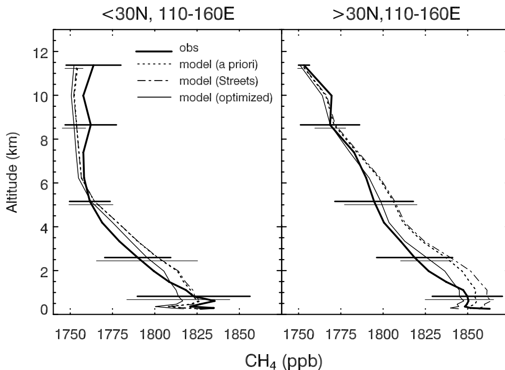
Figure 4b. Mean vertical profiles of CH 4 concentrations along the TRACE-P flight tracks, north of 30°N and south of 30°N at 110°E-160°E (NW Pacific, Asian outflow). Observations (thick lines) are compared to model values using the a priori emission inventory (dotted lines), the a priori inventory with anthropogenic East Asian sources from Streets et al. [2003] superimposed (dash-dotted lines), and the optimized emission inventory (solid lines). The a priori emission inventory is from Wang et al. [2003]. The optimized emission inventory uses East Asian anthropogenic emissions from Streets et al. [2003] and Eurasian anthropogenic emissions decreased by 50% from the Wang et al. [2003] inventory. The error bars show standard deviations ( 1\sigma ) for the observations and the optimized model at selected levels.
