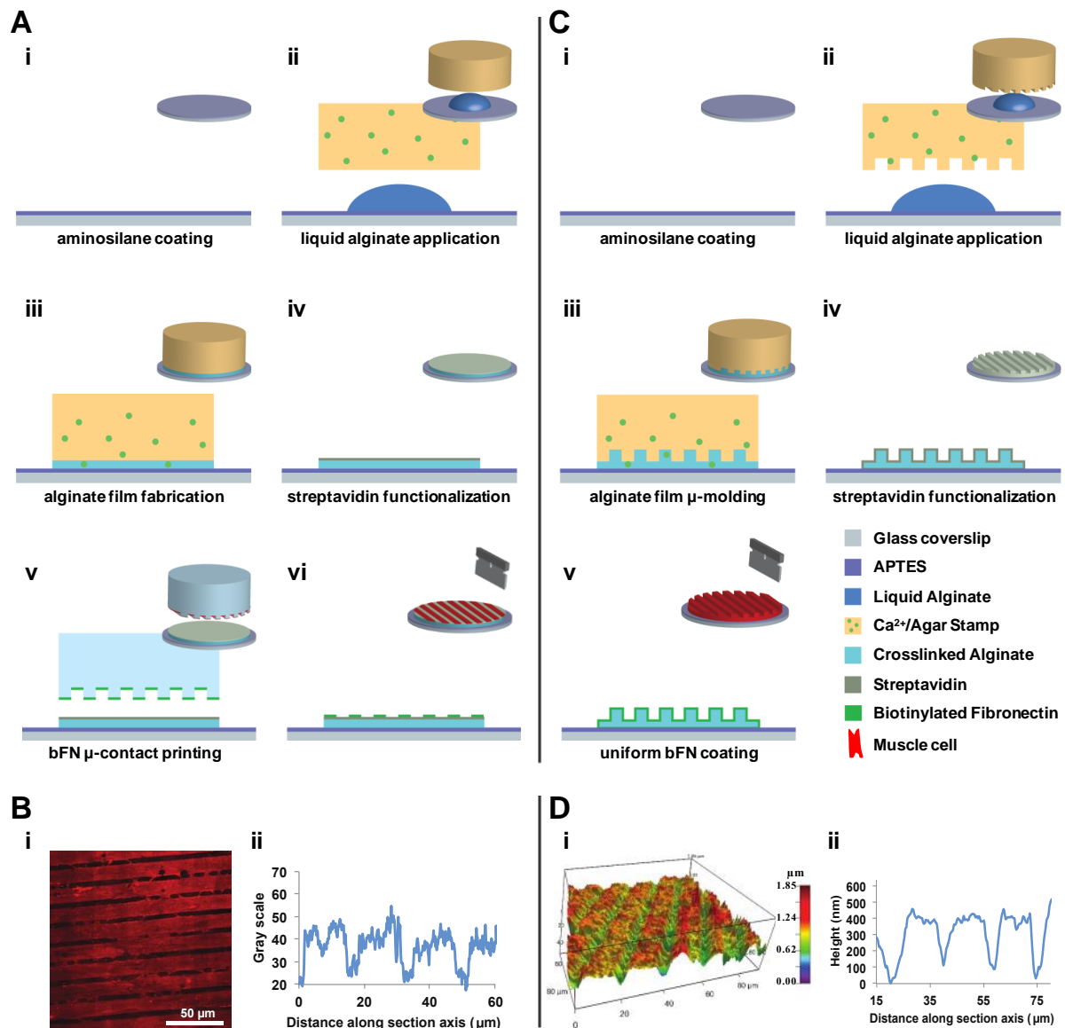
Figure 2. Micropatterned alginate thin films fabricated using (A, B) microcontact printing and (C, D) micromolding. (A, C i) A layer of APTES is deposited on the glass coverslip (A, C ii-iii) A flat or patterned calcium-loaded agar stamp is applied on a drop of alginate (A, C iv) The thin film of hydrogel is submerged in a solution of streptavidin mixed with the reagents EDC and Sulfo-NHS and then washed and dried (A, C v) Biotinylated fibronectin is applied either by microcontact printing with a stamp of PDMS or by simple submersion (A, C vi) Samples are ready for being cut for contractility assay. (B i) Fluorescent imaging of immunostained 2D fibronectin pattern on flat alginate films (B ii) Section profile of fluorescence level. (D i) 3D reconstruction of AFM imaging of the topography of micromolded films (D ii) Height profile along a section perpendicular to the features.
