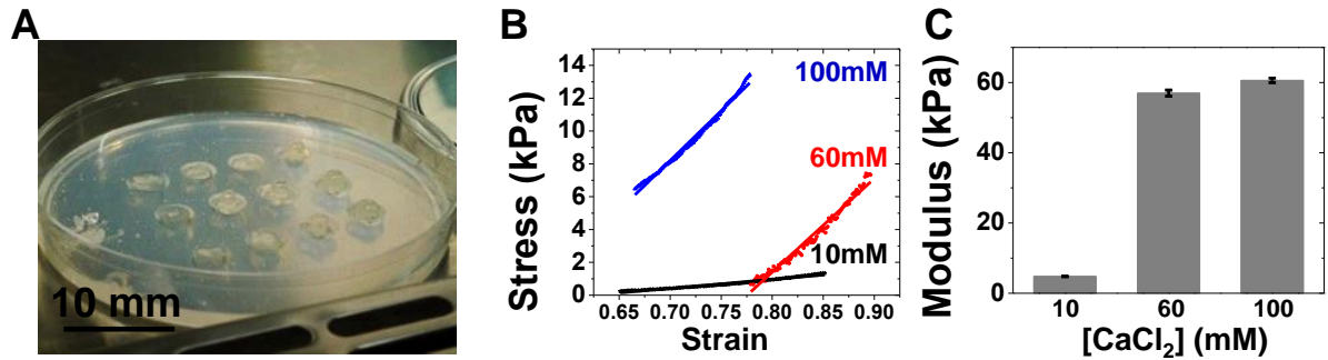
Figure 1. Mechanical characterization of 5% w/v of alginate. (A) Example photograph of 12 test samples punched out for mechanical testing. (B) Stress-strain curve collected for alginate substrates ionically crosslinked with 10mM, 60mM, and 100mM CaCl 2 . The straight line fits reveal a strong linear correlation implying elastic behavior. (C) Young's moduli for 10, 60, and 100mM CaCl 2 conditions calculated from the corresponding slope of the linear fits were determined to be 4.77 \pm 0.08 kPa, 56.98 \pm 0.86 kPa and 60.60 \pm 0.64 kPa respectively (Mean \pm SEM, N=3 samples).
