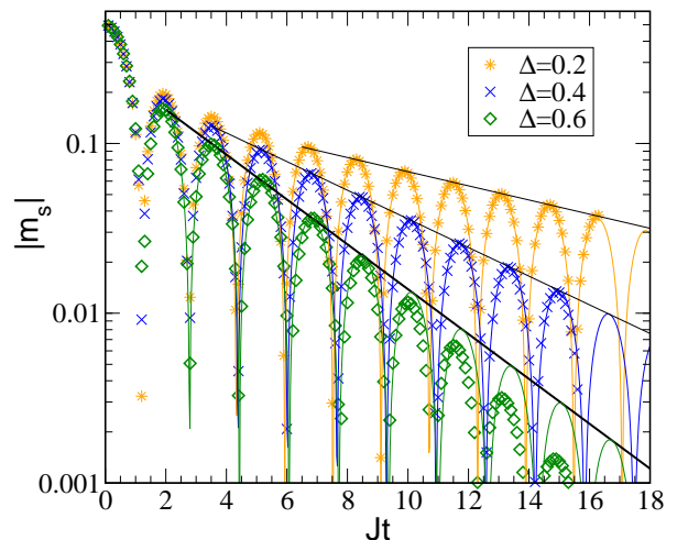
FIG. 3: Analysis of the decay of the oscillations in the XXZ model by plotting the absolute value of the staggered magnetization on a logarithmic scale. Symbols represent numerical results, solid curves correspond to fits by the function (27), straight lines point out the exponential decay. For anisotropies close to zero ( \Delta = 0.2, 0.4 ) an exponential law is obeyed for large periods of time in the numerically accessible time window, while for \Delta = 0.6 the simulation shows an acceleration of the decay after a few oscillations.
