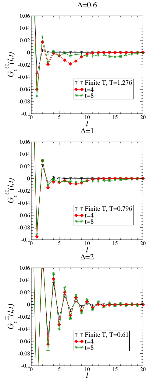
FIG. 6: The correlation functions obtained using iMPS for the initial Néel state. Symbols T denote quantum Monte Carlo results for the XXZ model at equilibrium at a temperature fixed by the energy of the non-equilibrium system.
