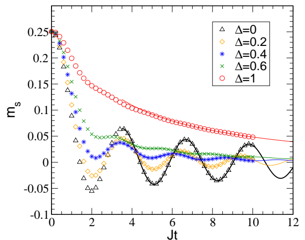
FIG. 8: Dynamics of the staggered magnetization m_s(t) in the XXZ chain prepared in an antiferromagnetic ground-state of the XXZ Hamiltonian with \Delta = \Delta_0 = 1.5 . Symbols correspond to numerical results, lines represent analytical results or fits by corresponding laws (29), (30) and (28) (see text).
