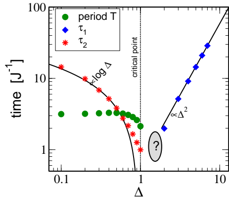
FIG. 4: Relaxation times and oscillation period T = \frac{2\pi}{\omega} as a function of anisotropy in the XXZ model for the Néel initial state. Logarithmic or algebraic laws are emphasized by solid lines. In the region close to the critical point of the XXZ model (indicated by the question mark) it becomes impossible to extract a relaxation time from the numerical results.
