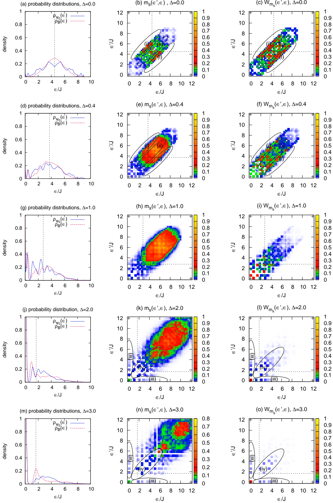
FIG. 13: Analysis of the spectrum of the XXZ chain for a system of 14 sites with periodic boundary conditions. Dotted lines mark the position of the energy of the system, E = \langle \psi_0 | H | \psi_0 \rangle . See text for the description of the regions marked (i)-(iv).
