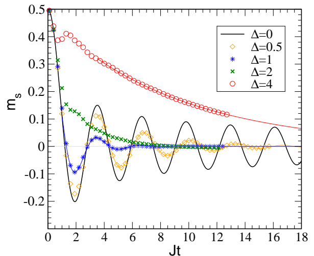
FIG. 2: Dynamics of the staggered magnetization m_s(t) in the XXZ chain initialized in a Néel state. Symbols correspond to numerical results, lines represent analytical results or fits by corresponding laws (27) and (28) (see text).
