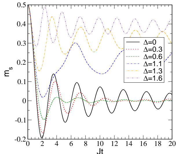
FIG. 10: Numerical solution of the mean field equations for the Hamiltonian (32) with the initial condition m_s(0) = \frac{1}{2} .
