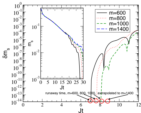
FIG. 19: The absolute error (C29) in an iMPS simulation for \delta = 0.005 , \epsilon = 10^{-17} for different values of m . Inset: the corresponding dynamics of m_s(t) .
