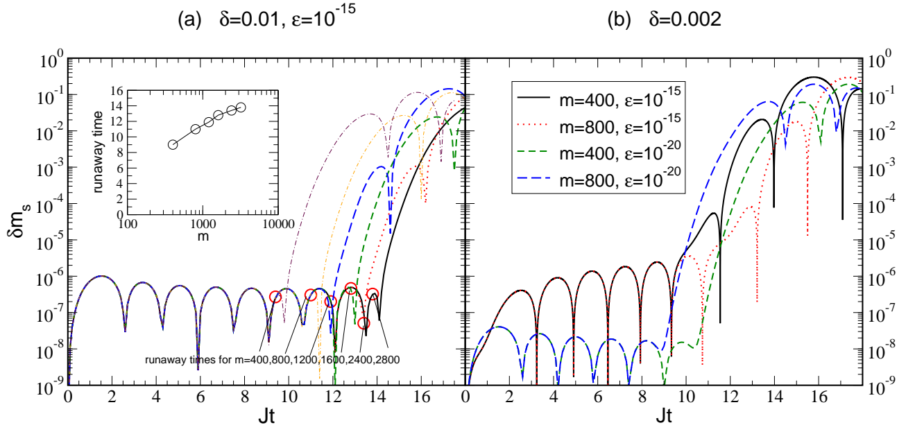
FIG. 18: The error in an iMPS compared to the exact solution. (a) Trotter slicing \delta = 0.01 , threshold \epsilon = 10^{-15} . Inset: runaway times as a function of m . (b) Comparison of errors for two different \epsilon = 10^{-15}, 10^{-20} , for a smaller slicing \delta = 0.002 .
