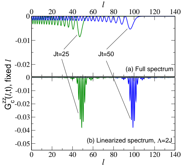
FIG. 1: Correlation functions in the XX limit. Comparison of results obtained for full (a) and linearized (b) spectra. For the linearized spectrum we set \Lambda = 2J as the effective bandwidth.
