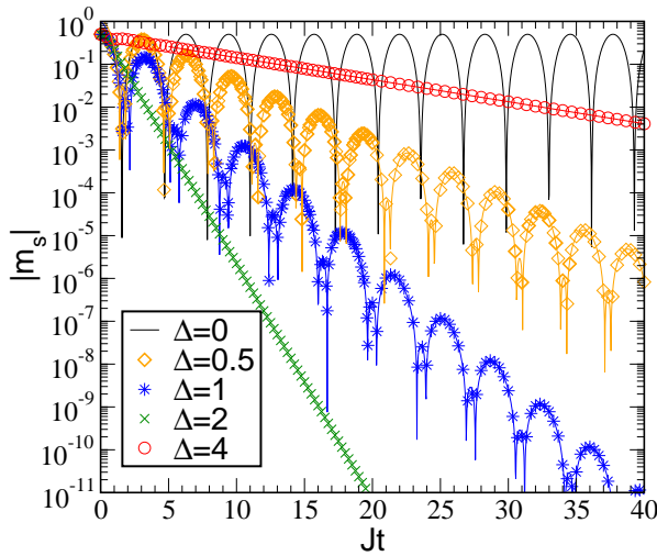
FIG. 11: Dynamics of the staggered magnetization m_s(t) in the XZ chain initialized in a Néel state. Symbols correspond to numerical results, lines represent analytical results or fits by corresponding laws (see text).
