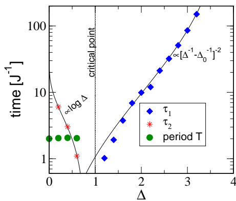
FIG. 7: Relaxation times and oscillation period T = \frac{2\pi}{\omega} as a function of anisotropy in the XXZ model for the system prepared in the ground state for \Delta_0 = 4 . Logarithmic or algebraic laws are emphasized by solid lines.
