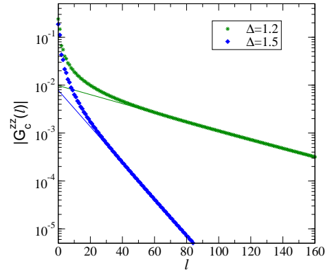
FIG. 17: Correlation function in the ground state at \Delta = 1.2, 1.5 . Straight lines are exponential laws e^{-\ell/\xi} . While for \Delta = 1.5 the inverse correlation length \xi^{-1} = 0.0873 is very close to the value predicted by the Klein-Gordon model ( \Delta_s/J = 0.0866 ), for \Delta = 1.2 it is considerably larger ( \xi^{-1} = 0.021 , \Delta_s/J = 0.0048 ).
