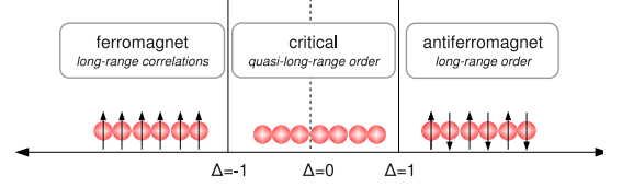
FIG. 15: The ground-state phase diagram of the XXZ model in one dimension.
