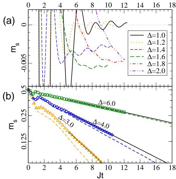
FIG. 5: (a) Focus on the XXZ chain close to the critical point \Delta = 1 , where a steep decay of the initial magnetization is followed by a rather slow relaxation on tiny magnitudes which does not fit either of the generic behaviors (27,28). (b) Comparison of the XXZ chain (symbols) and the XZ chain (dashed lines) for strong anisotropies, solid lines correspond to an exponential fit. The dynamics of the staggered magnetization of the XXZ and XZ chains converge towards each other in the large- \Delta limit.
