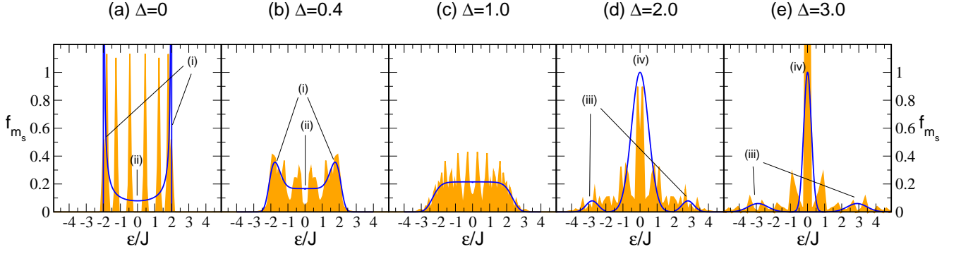
FIG. 14: The frequency distribution of the staggered magnetization, f_{m_s}(\epsilon) , for a system of 14 sites with periodic boundary conditions. Histograms resolve individual peaks, solid lines correspond to (non-unique) smoothed distributions emphasizing separable contributions. For \Delta = 0 the exact solution in the thermodynamic limit (14) is drawn instead.
