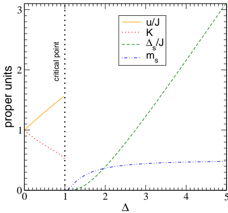
FIG. 16: The Luttinger parameter K , the velocity u , the gap \Delta_s , and the staggered magnetization m_s in the XXZ model, calculated by Bethe ansatz.
