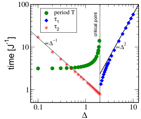
FIG. 12: Relaxation times and oscillation period T = \frac{2\pi}{\omega} as a function of anisotropy in the XZ model. Algebraic laws are emphasized by solid lines.
